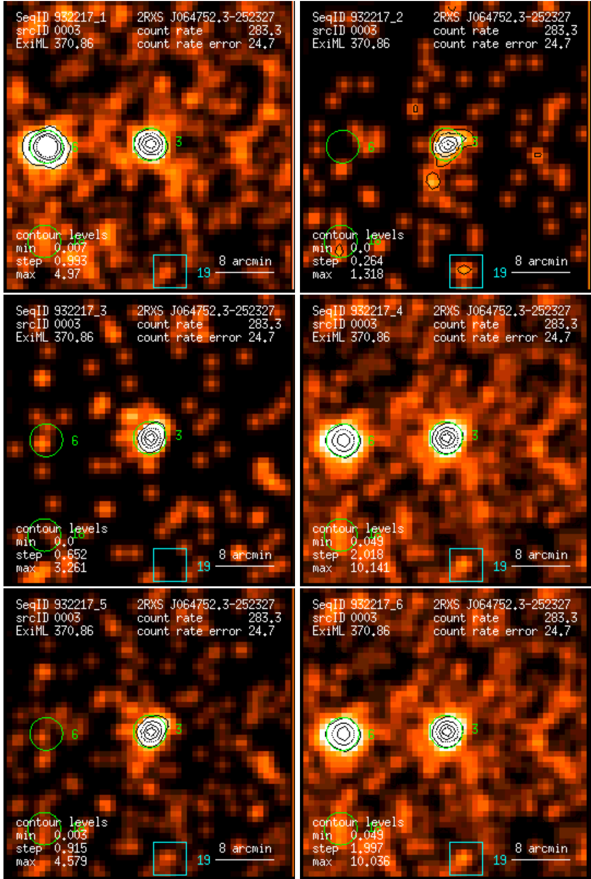
Figure 3: RASS 932217: detection 0003: band rate images, Gaussian filter: (1) PSPC channels 11 – 41, (2) 52 – 90, (3) 91 – 201, (4) 11 – 235, (5) 52 – 201, (6) 11 – 201. Broad band rates in counts/ks. Band rate contour levels in counts/ks/arcmin 2 .
