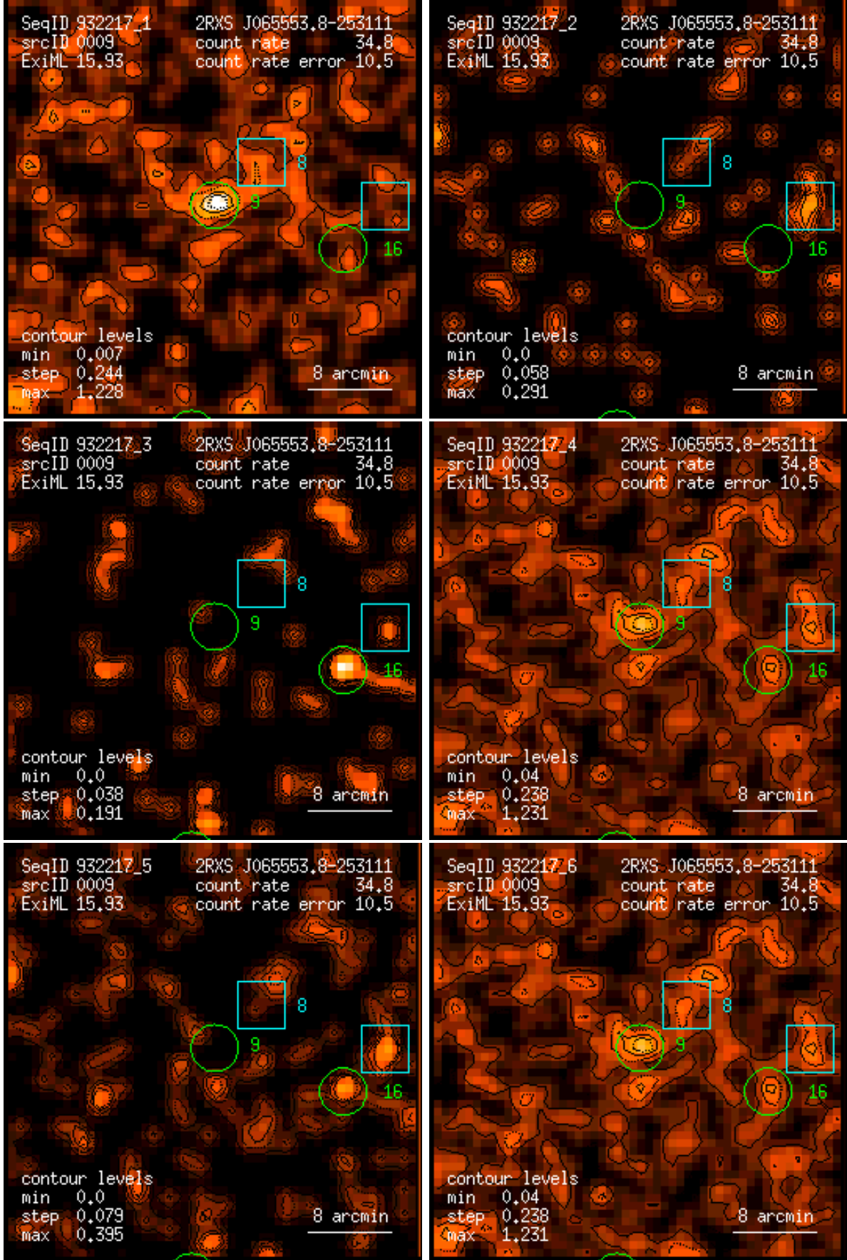
Figure 9: RASS 932217: detection 0009: band rate images, Gaussian filter: (1) PSPC channels 11 – 41, (2) 52 – 90, (3) 91 – 201, (4) 11 – 235, (5) 52 – 201, (6) 11 – 201. Broad band rates in counts/ks. Band rate contour levels in counts/ks/arcmin 2 .
