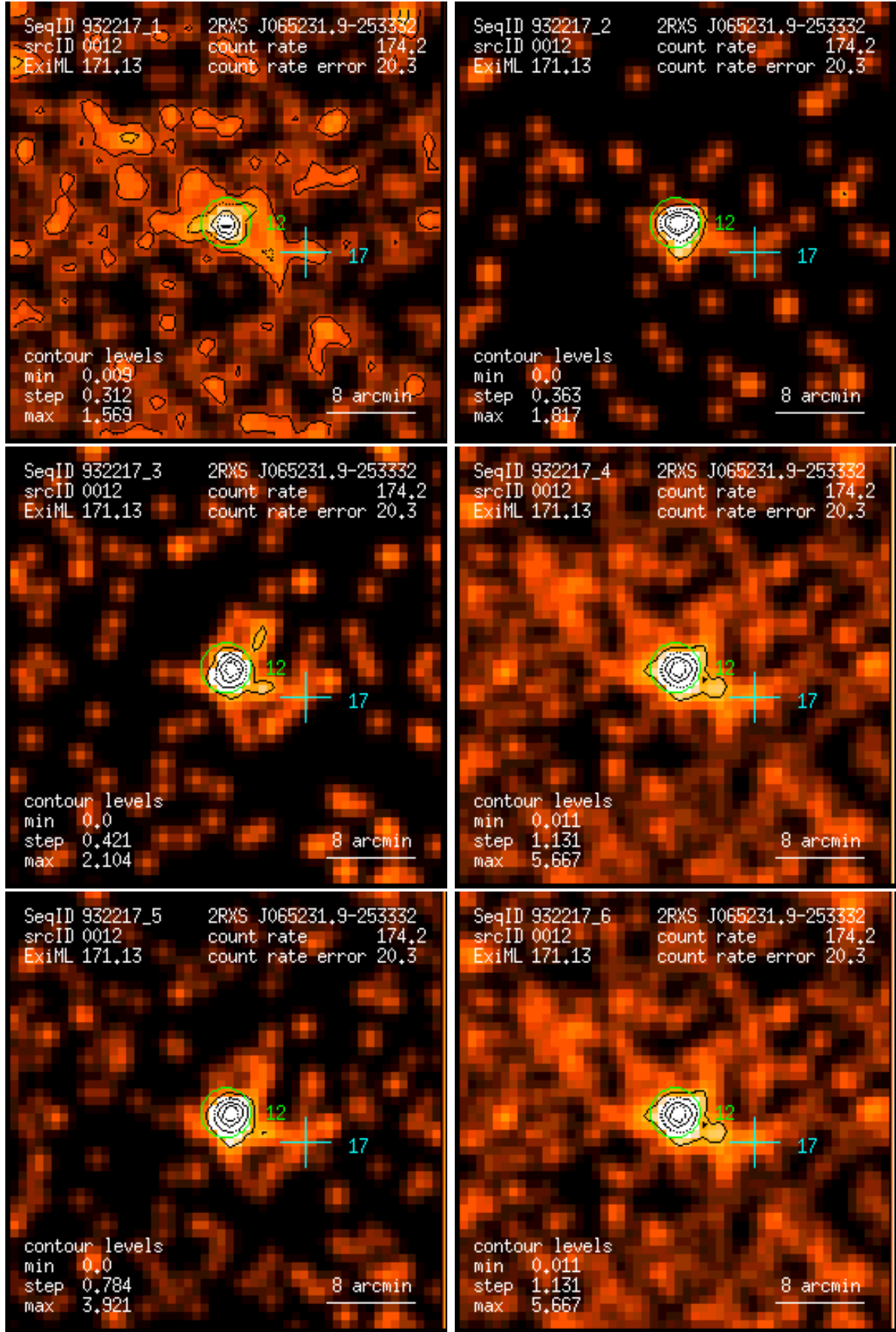
Figure 12: RASS 932217: detection 0012: band rate images, Gaussian filter: (1) PSPC channels 11 – 41, (2) 52 – 90, (3) 91 – 201, (4) 11 – 235, (5) 52 – 201, (6) 11 – 201. Broad band rates in counts/ks. Band rate contour levels in counts/ks/arcmin 2 .
