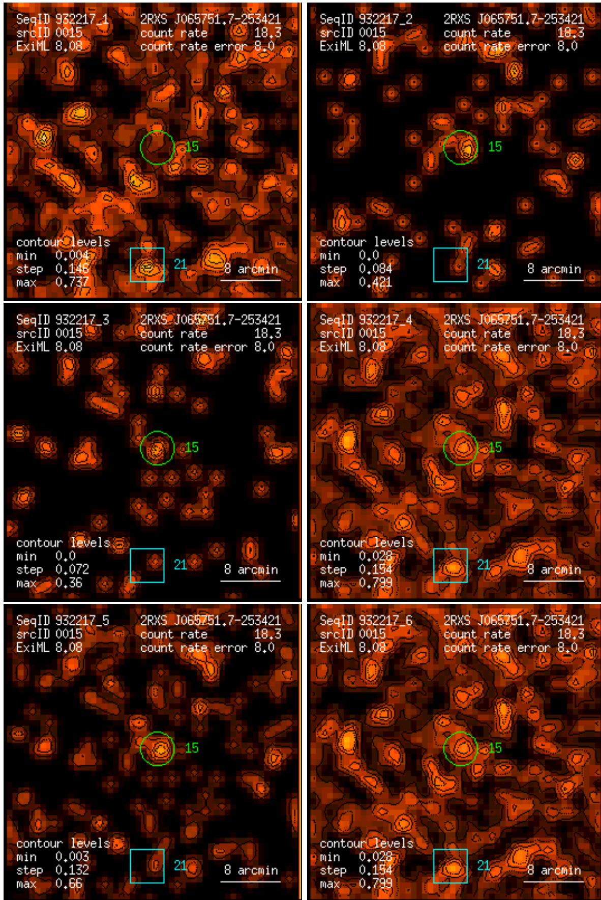
Figure 15: RASS 932217: detection 0015: band rate images, Gaussian filter: (1) PSPC channels 11 – 41, (2) 52 – 90, (3) 91 – 201, (4) 11 – 235, (5) 52 – 201, (6) 11 – 201. Broad band rates in counts/ks. Band rate contour levels in counts/ks/arcmin 2 .
