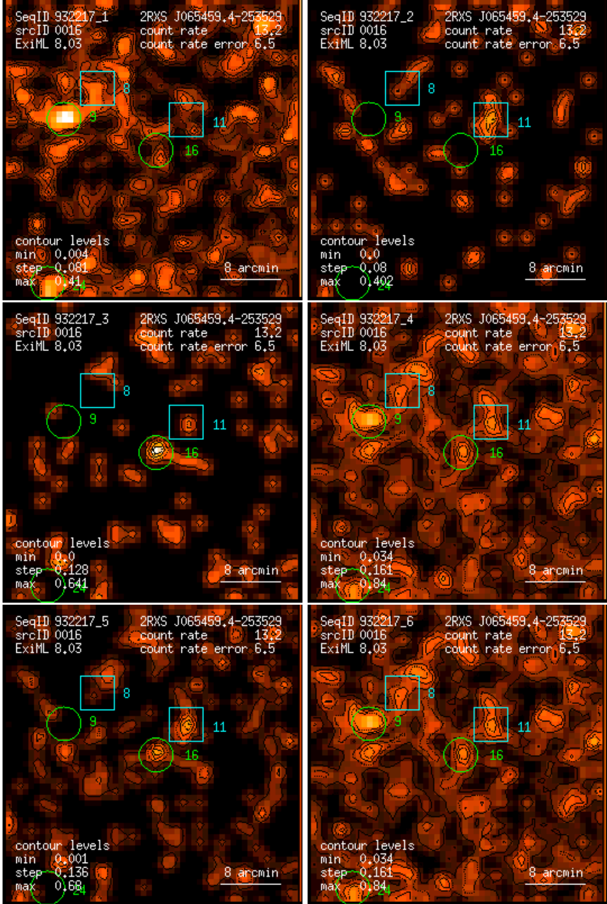
Figure 16: RASS 932217: detection 0016: band rate images, Gaussian filter: (1) PSPC channels 11 – 41, (2) 52 – 90, (3) 91 – 201, (4) 11 – 235, (5) 52 – 201, (6) 11 – 201. Broad band rates in counts/ks. Band rate contour levels in counts/ks/arcmin 2 .
