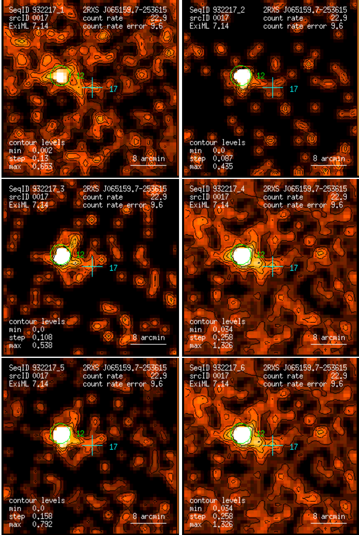
Figure 17: RASS 932217: detection 0017: band rate images, Gaussian filter: (1) PSPC channels 11 – 41, (2) 52 – 90, (3) 91 – 201, (4) 11 – 235, (5) 52 – 201, (6) 11 – 201. Broad band rates in counts/ks. Band rate contour levels in counts/ks/arcmin 2 .
