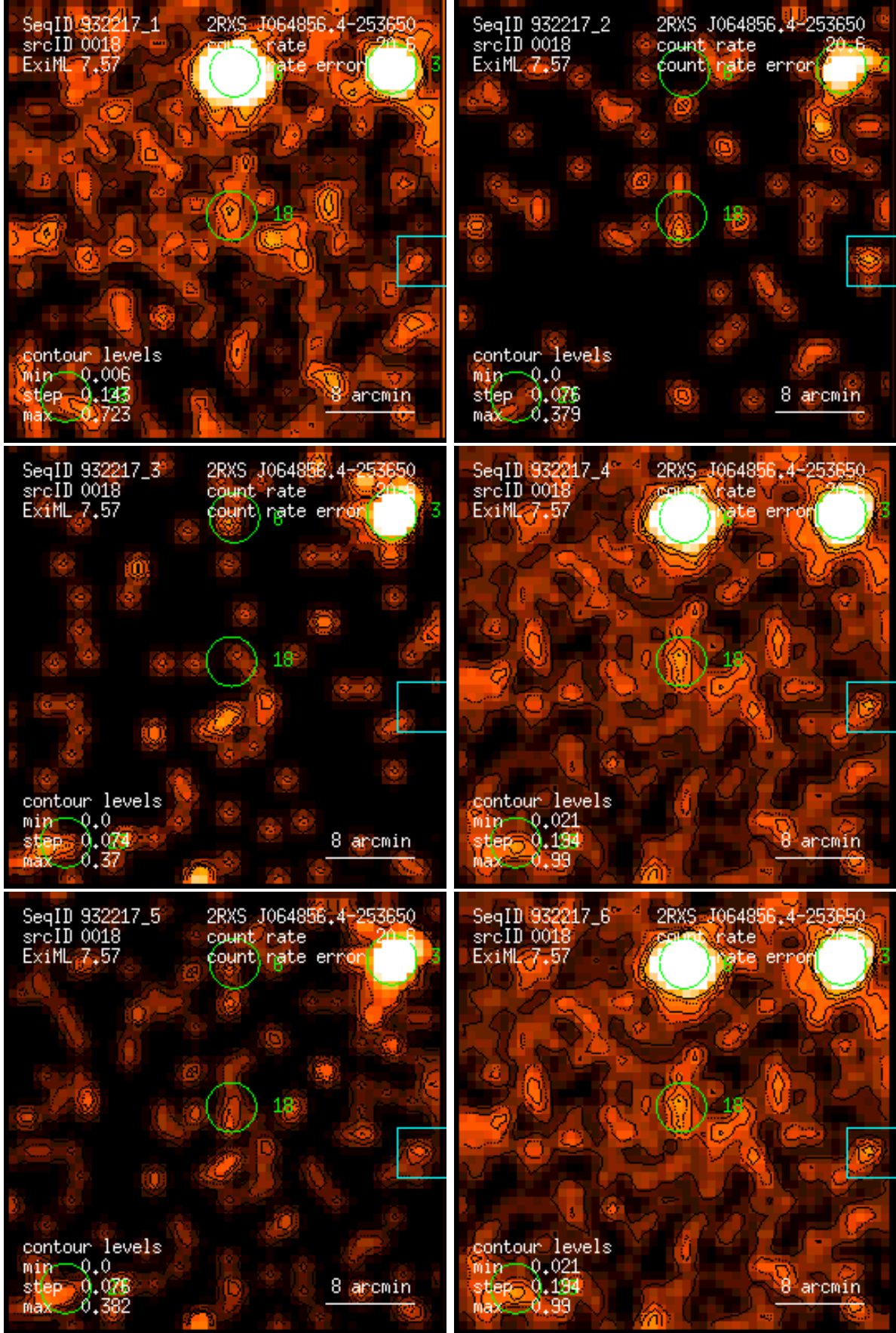
Figure 18: RASS 932217: detection 0018: band rate images, Gaussian filter: (1) PSPC channels 11 – 41, (2) 52 – 90, (3) 91 – 201, (4) 11 – 235, (5) 52 – 201, (6) 11 – 201. Broad band rates in counts/ks. Band rate contour levels in counts/ks/arcmin 2 .
