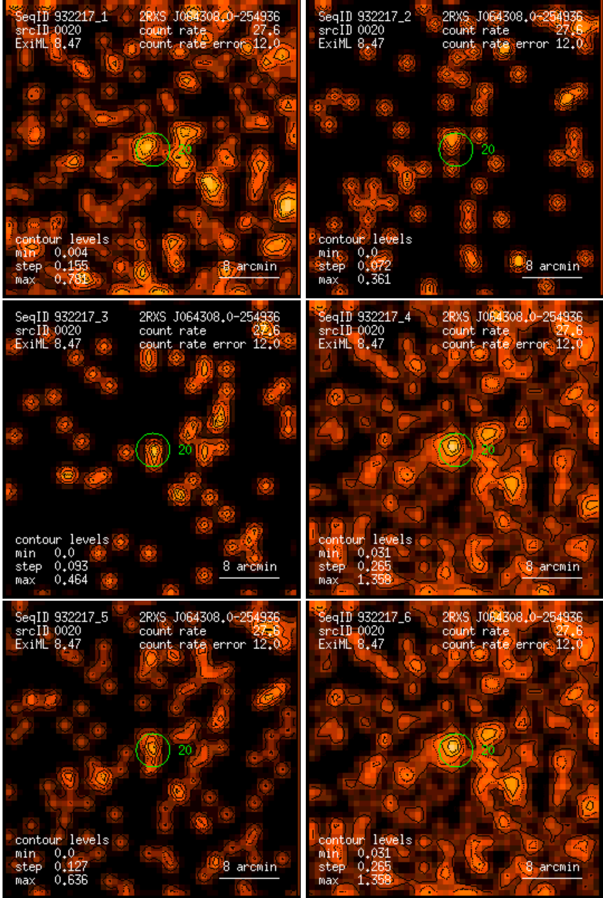
Figure 20: RASS 932217: detection 0020: band rate images, Gaussian filter: (1) PSPC channels 11 – 41, (2) 52 – 90, (3) 91 – 201, (4) 11 – 235, (5) 52 – 201, (6) 11 – 201. Broad band rates in counts/ks. Band rate contour levels in counts/ks/arcmin 2 .
