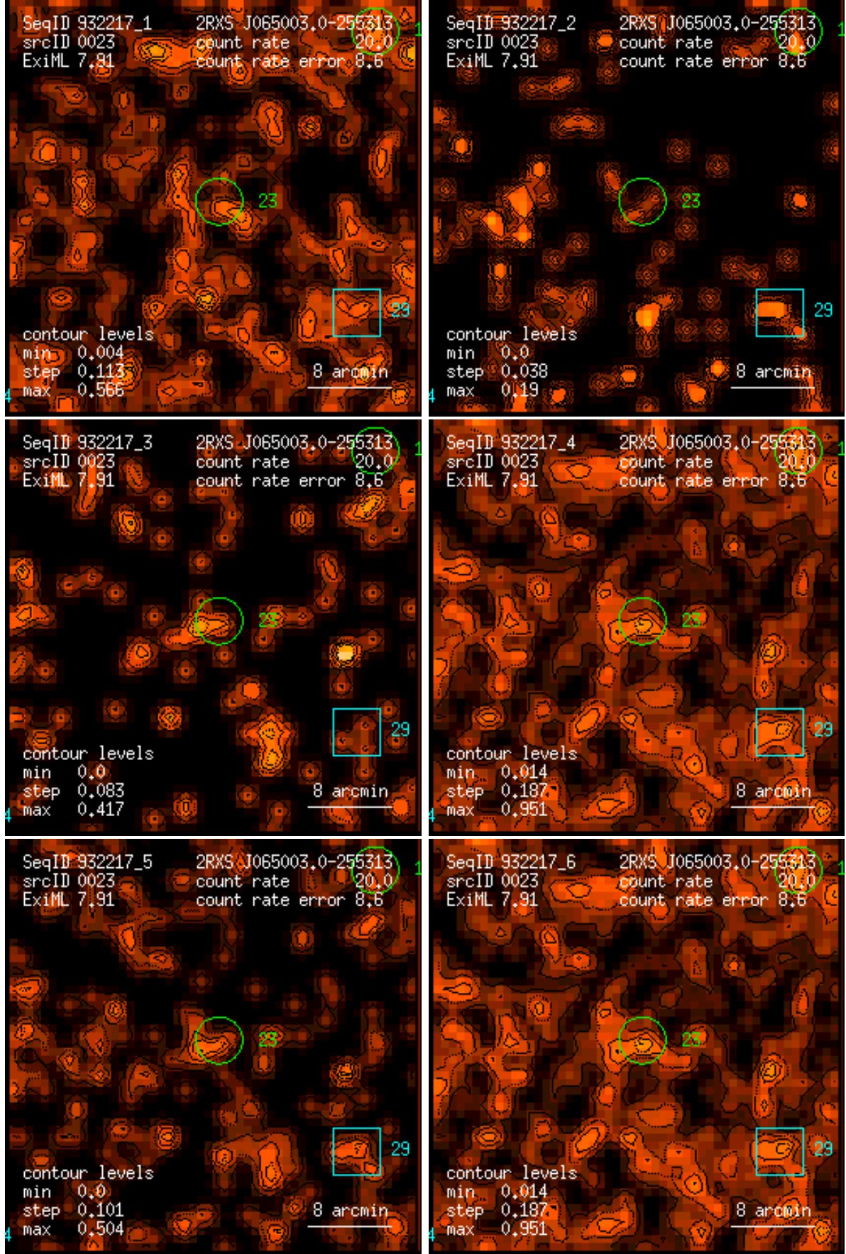
Figure 23: RASS 932217: detection 0023: band rate images, Gaussian filter: (1) PSPC channels 11 – 41, (2) 52 – 90, (3) 91 – 201, (4) 11 – 235, (5) 52 – 201, (6) 11 – 201. Broad band rates in counts/ks. Band rate contour levels in counts/ks/arcmin 2 .
