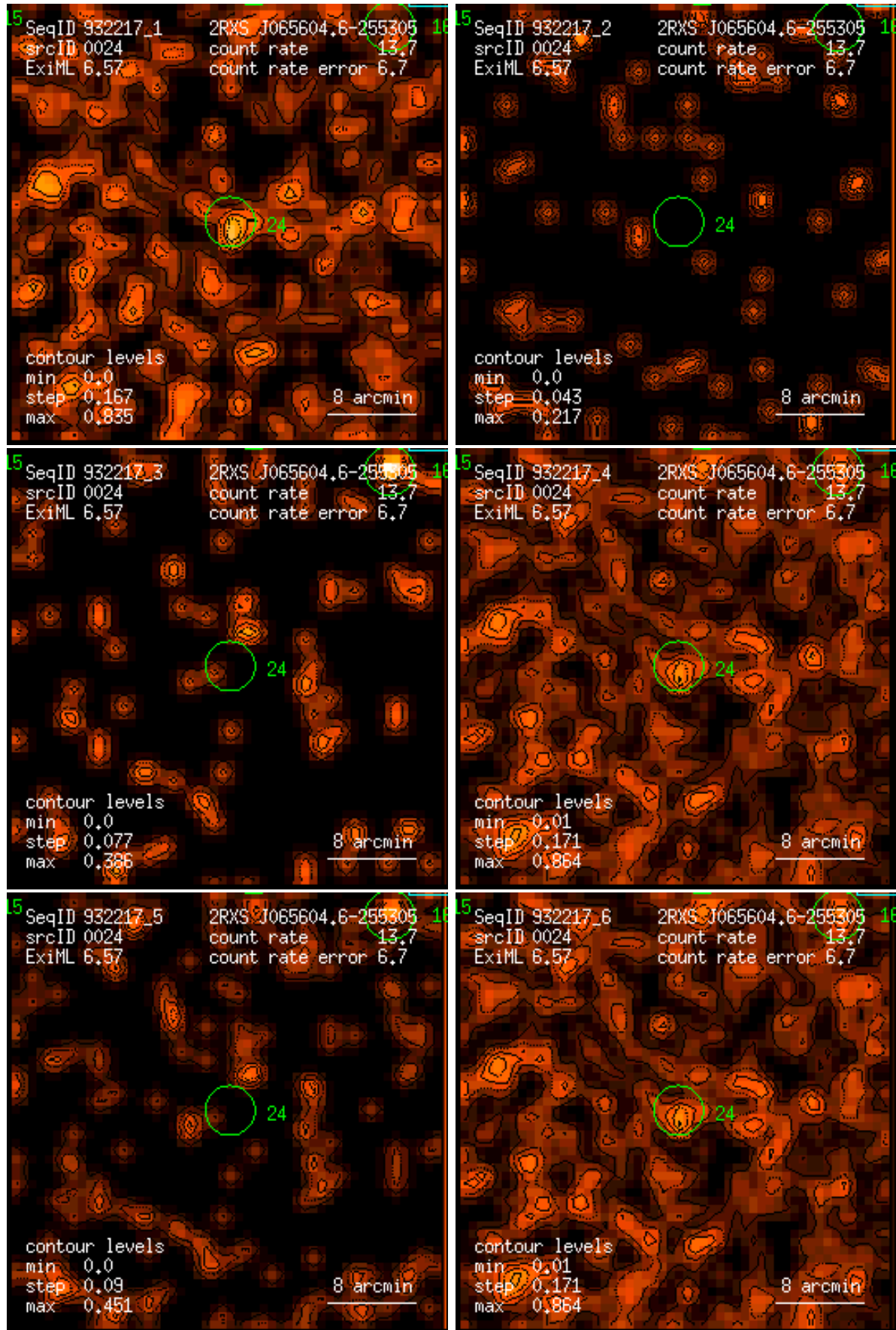
Figure 24: RASS 932217: detection 0024: band rate images, Gaussian filter: (1) PSPC channels 11 – 41, (2) 52 – 90, (3) 91 – 201, (4) 11 – 235, (5) 52 – 201, (6) 11 – 201. Broad band rates in counts/ks. Band rate contour levels in counts/ks/arcmin 2 .
