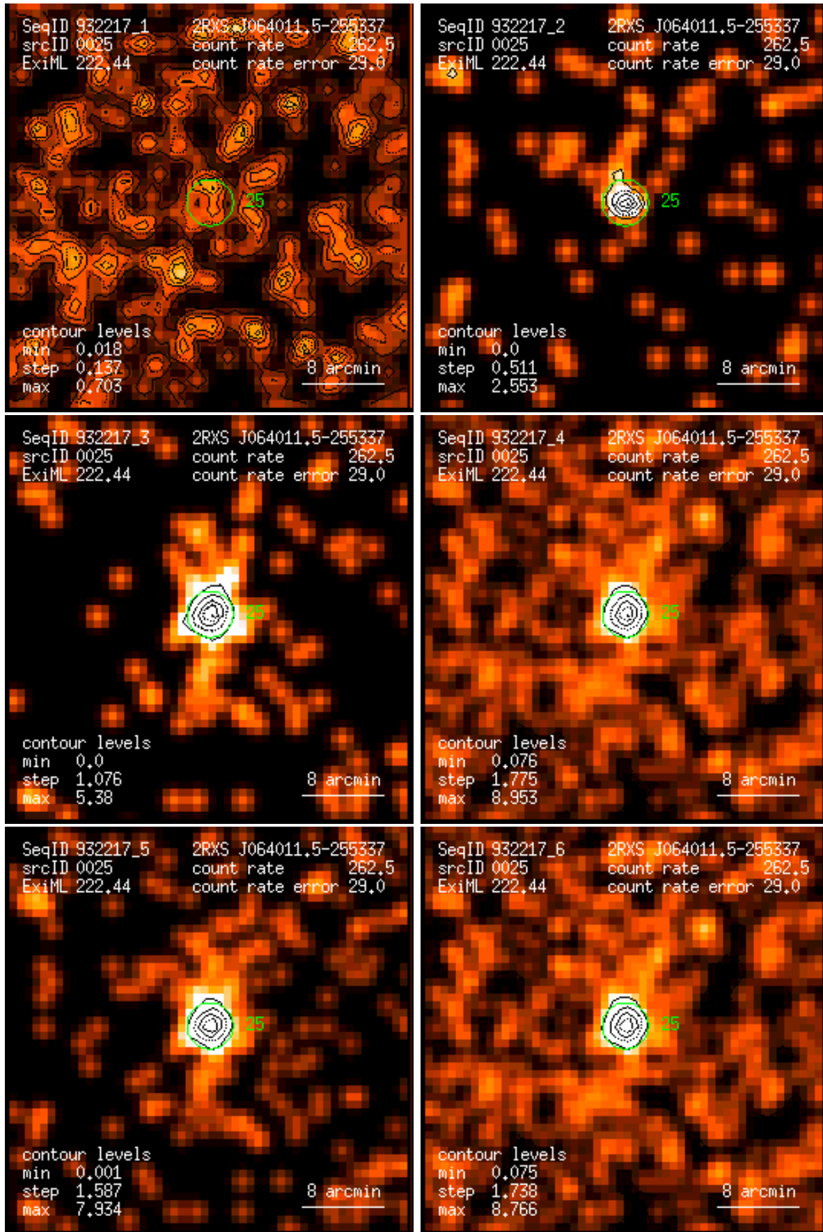
Figure 25: RASS 932217: detection 0025: band rate images, Gaussian filter: (1) PSPC channels 11 – 41, (2) 52 – 90, (3) 91 – 201, (4) 11 – 235, (5) 52 – 201, (6) 11 – 201. Broad band rates in counts/ks. Band rate contour levels in counts/ks/arcmin 2 .
