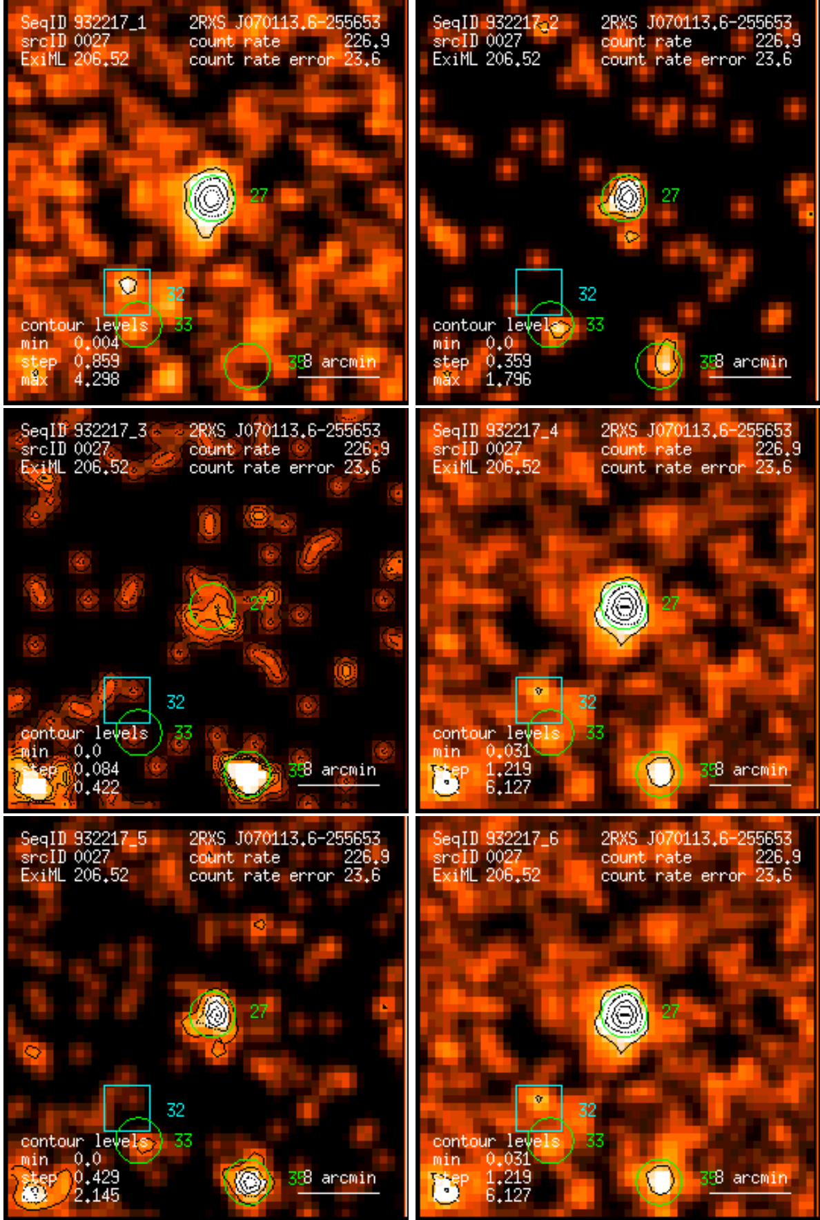
Figure 27: RASS 932217: detection 0027: band rate images, Gaussian filter: (1) PSPC channels 11 – 41, (2) 52 – 90, (3) 91 – 201, (4) 11 – 235, (5) 52 – 201, (6) 11 – 201. Broad band rates in counts/ks. Band rate contour levels in counts/ks/arcmin 2 .
