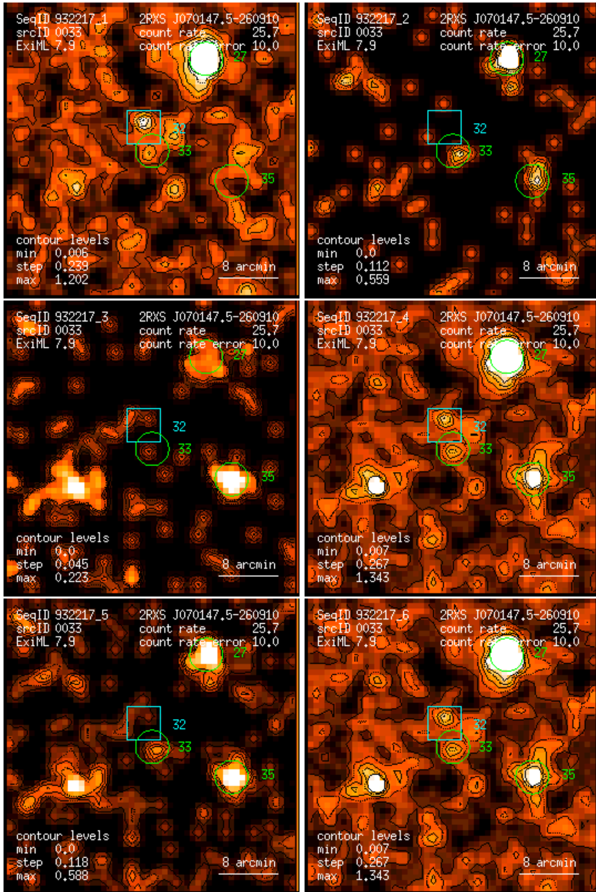
Figure 33: RASS 932217: detection 0033: band rate images, Gaussian filter: (1) PSPC channels 11 – 41, (2) 52 – 90, (3) 91 – 201, (4) 11 – 235, (5) 52 – 201, (6) 11 – 201. Broad band rates in counts/ks. Band rate contour levels in counts/ks/arcmin 2 .
