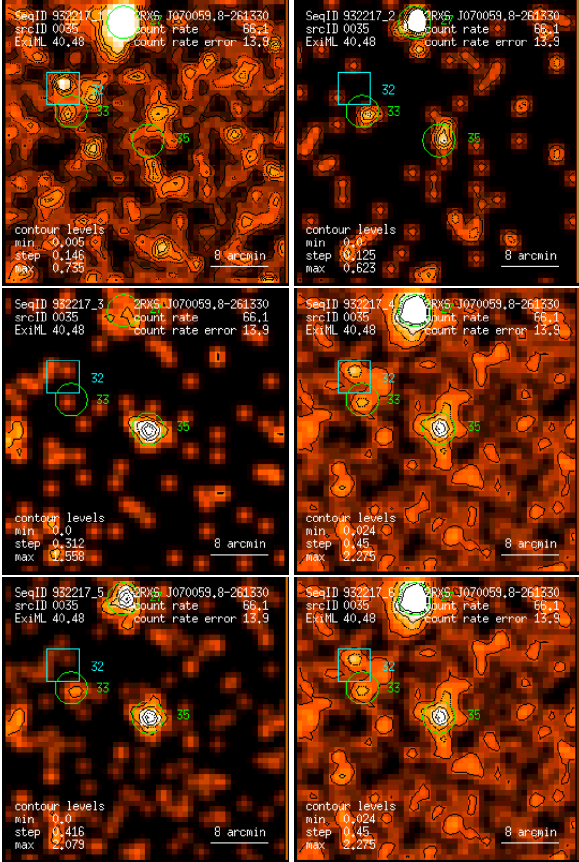
Figure 35: RASS 932217: detection 0035: band rate images, Gaussian filter: (1) PSPC channels 11 – 41, (2) 52 – 90, (3) 91 – 201, (4) 11 – 235, (5) 52 – 201, (6) 11 – 201. Broad band rates in counts/ks. Band rate contour levels in counts/ks/arcmin 2 .
