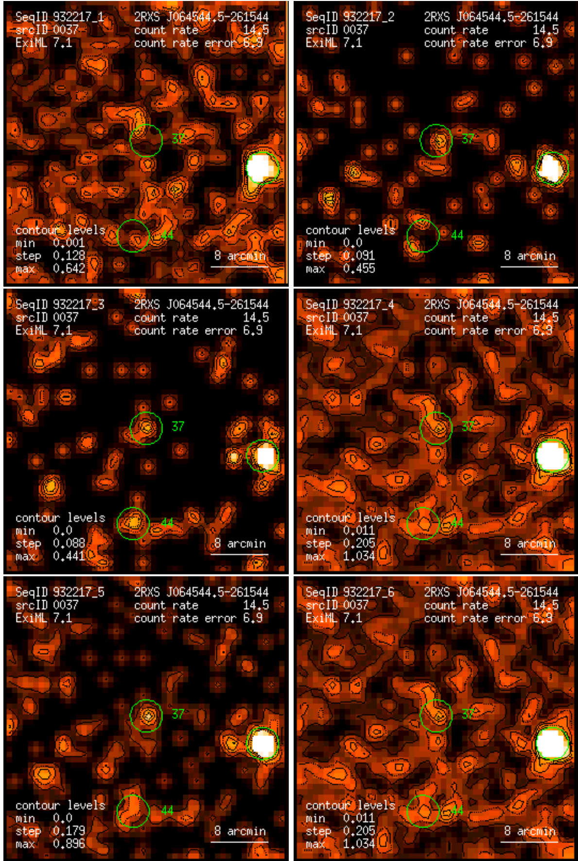
Figure 37: RASS 932217: detection 0037: band rate images, Gaussian filter: (1) PSPC channels 11 – 41, (2) 52 – 90, (3) 91 – 201, (4) 11 – 235, (5) 52 – 201, (6) 11 – 201. Broad band rates in counts/ks. Band rate contour levels in counts/ks/arcmin 2 .
