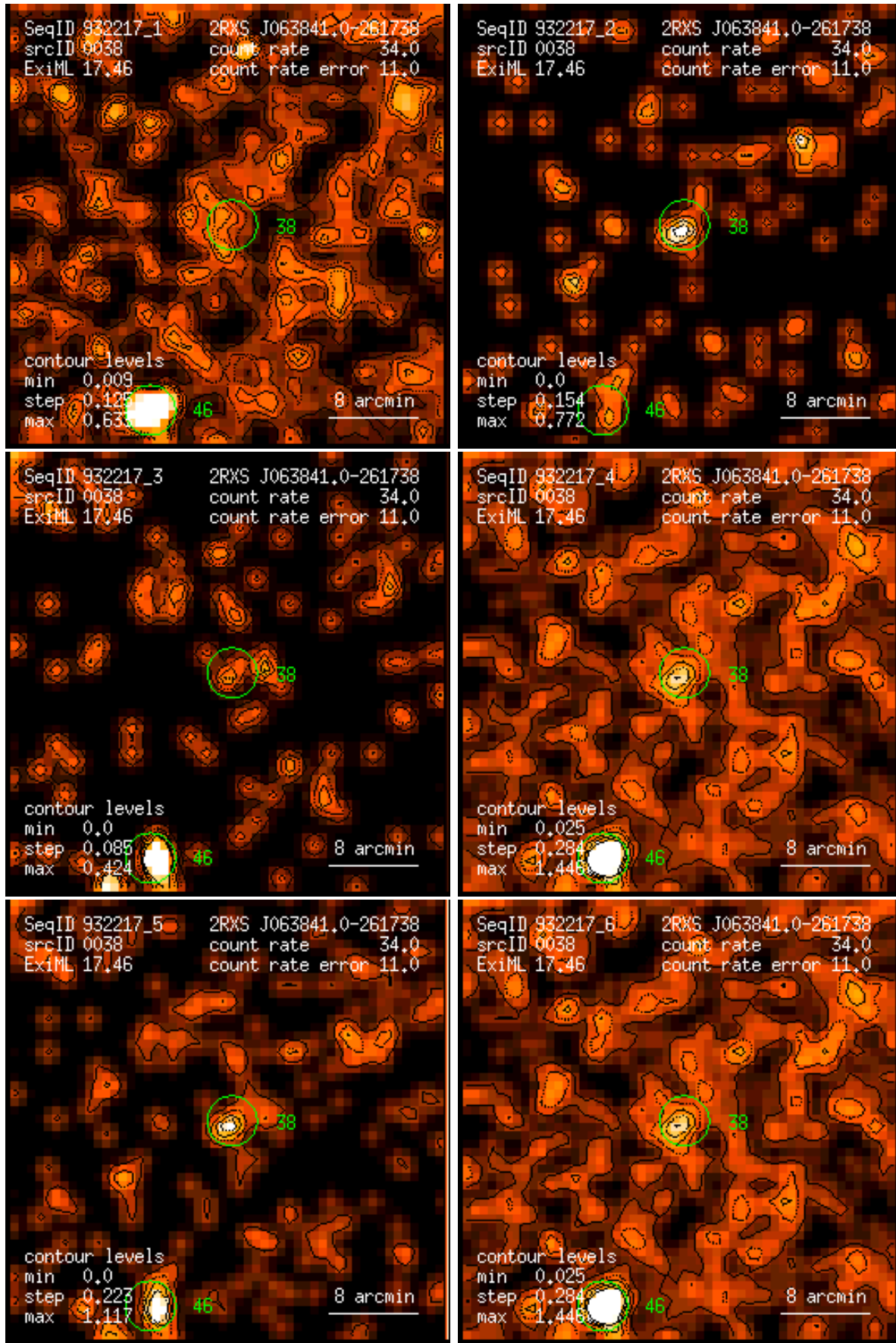
Figure 38: RASS 932217: detection 0038: band rate images, Gaussian filter: (1) PSPC channels 11 – 41, (2) 52 – 90, (3) 91 – 201, (4) 11 – 235, (5) 52 – 201, (6) 11 – 201. Broad band rates in counts/ks. Band rate contour levels in counts/ks/arcmin 2 .
