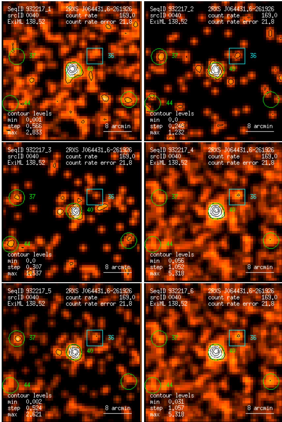
Figure 40: RASS 932217: detection 0040: band rate images, Gaussian filter: (1) PSPC channels 11 – 41, (2) 52 – 90, (3) 91 – 201, (4) 11 – 235, (5) 52 – 201, (6) 11 – 201. Broad band rates in counts/ks. Band rate contour levels in counts/ks/arcmin 2 .
