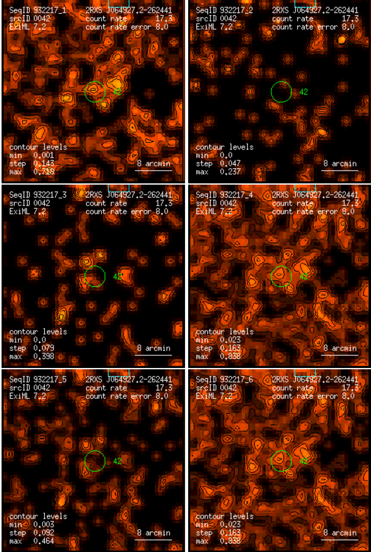
Figure 42: RASS 932217: detection 0042: band rate images, Gaussian filter: (1) PSPC channels 11 – 41, (2) 52 – 90, (3) 91 – 201, (4) 11 – 235, (5) 52 – 201, (6) 11 – 201. Broad band rates in counts/ks. Band rate contour levels in counts/ks/arcmin 2 .
