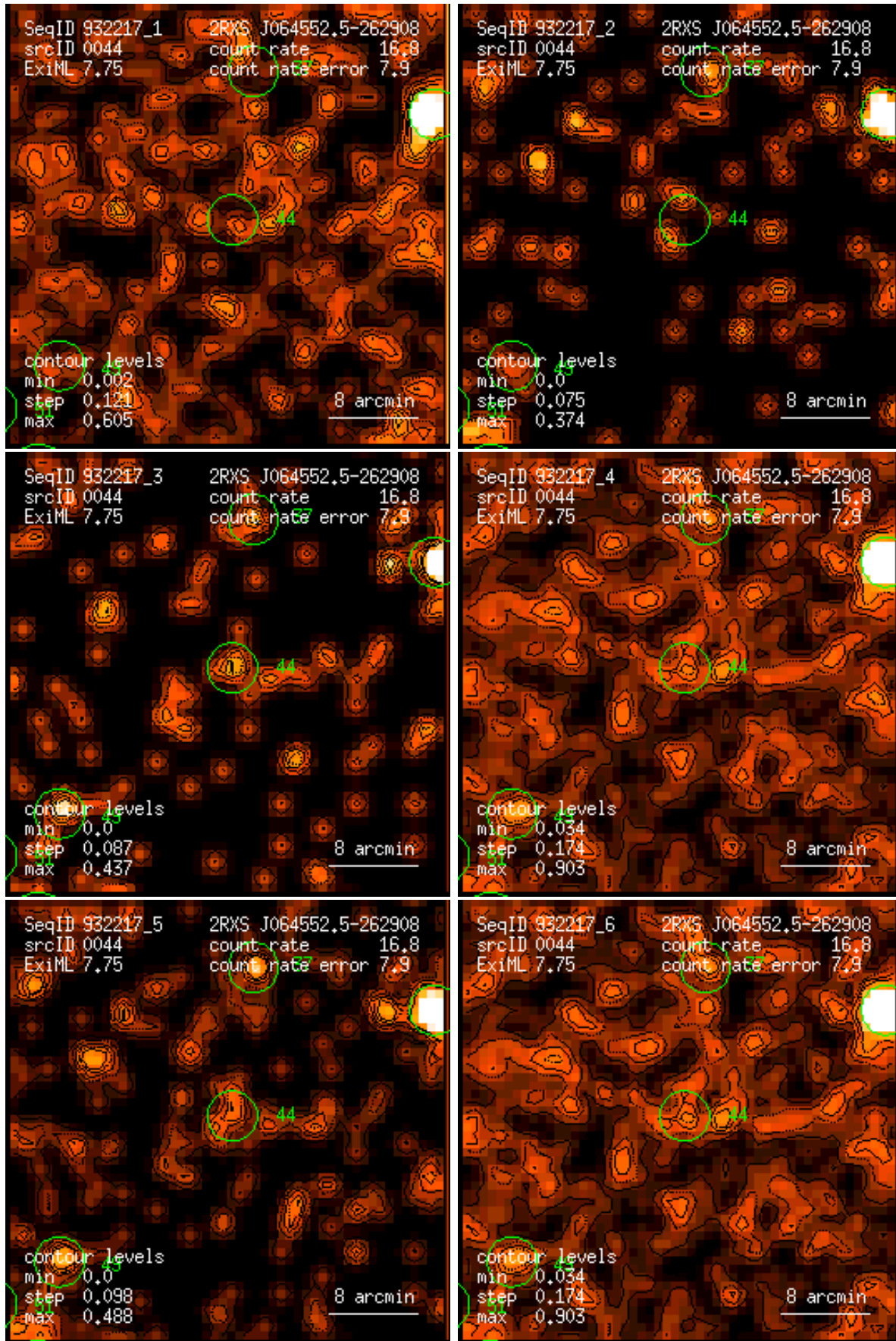
Figure 44: RASS 932217: detection 0044: band rate images, Gaussian filter: (1) PSPC channels 11 – 41, (2) 52 – 90, (3) 91 – 201, (4) 11 – 235, (5) 52 – 201, (6) 11 – 201. Broad band rates in counts/ks. Band rate contour levels in counts/ks/arcmin 2 .
