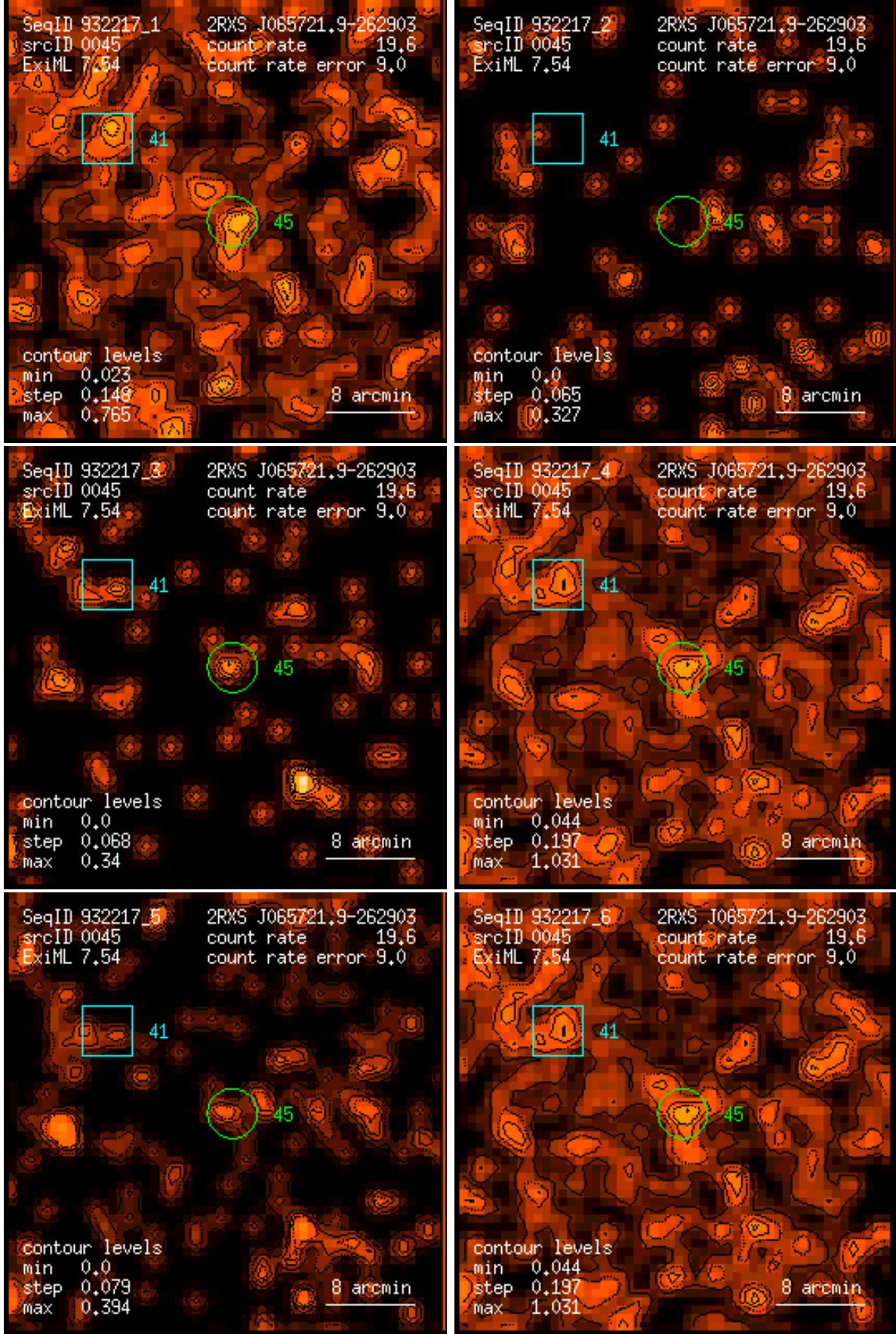
Figure 45: RASS 932217: detection 0045: band rate images, Gaussian filter: (1) PSPC channels 11 – 41, (2) 52 – 90, (3) 91 – 201, (4) 11 – 235, (5) 52 – 201, (6) 11 – 201. Broad band rates in counts/ks. Band rate contour levels in counts/ks/arcmin 2 .
