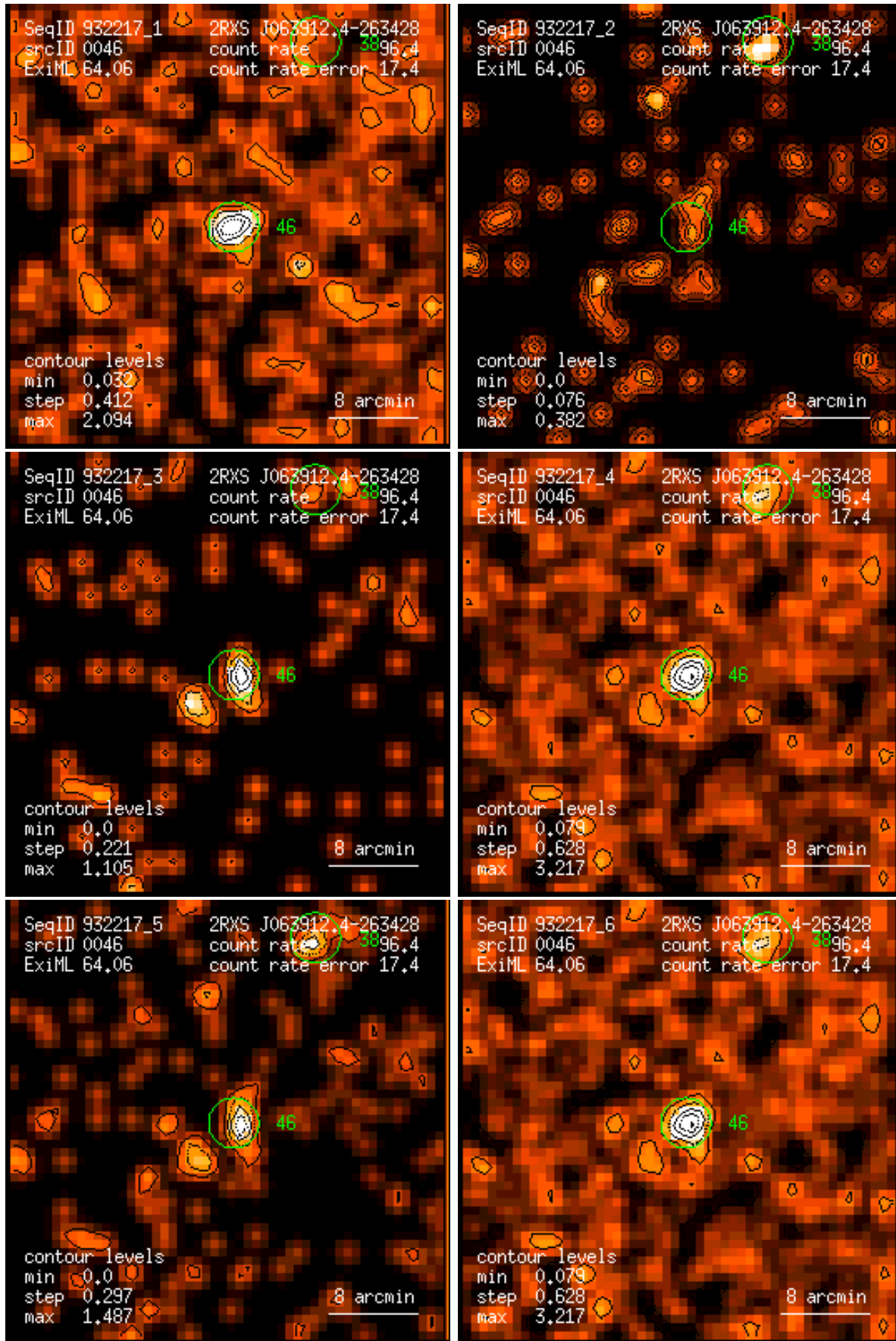
Figure 46: RASS 932217: detection 0046: band rate images, Gaussian filter: (1) PSPC channels 11 – 41, (2) 52 – 90, (3) 91 – 201, (4) 11 – 235, (5) 52 – 201, (6) 11 – 201. Broad band rates in counts/ks. Band rate contour levels in counts/ks/arcmin 2 .
