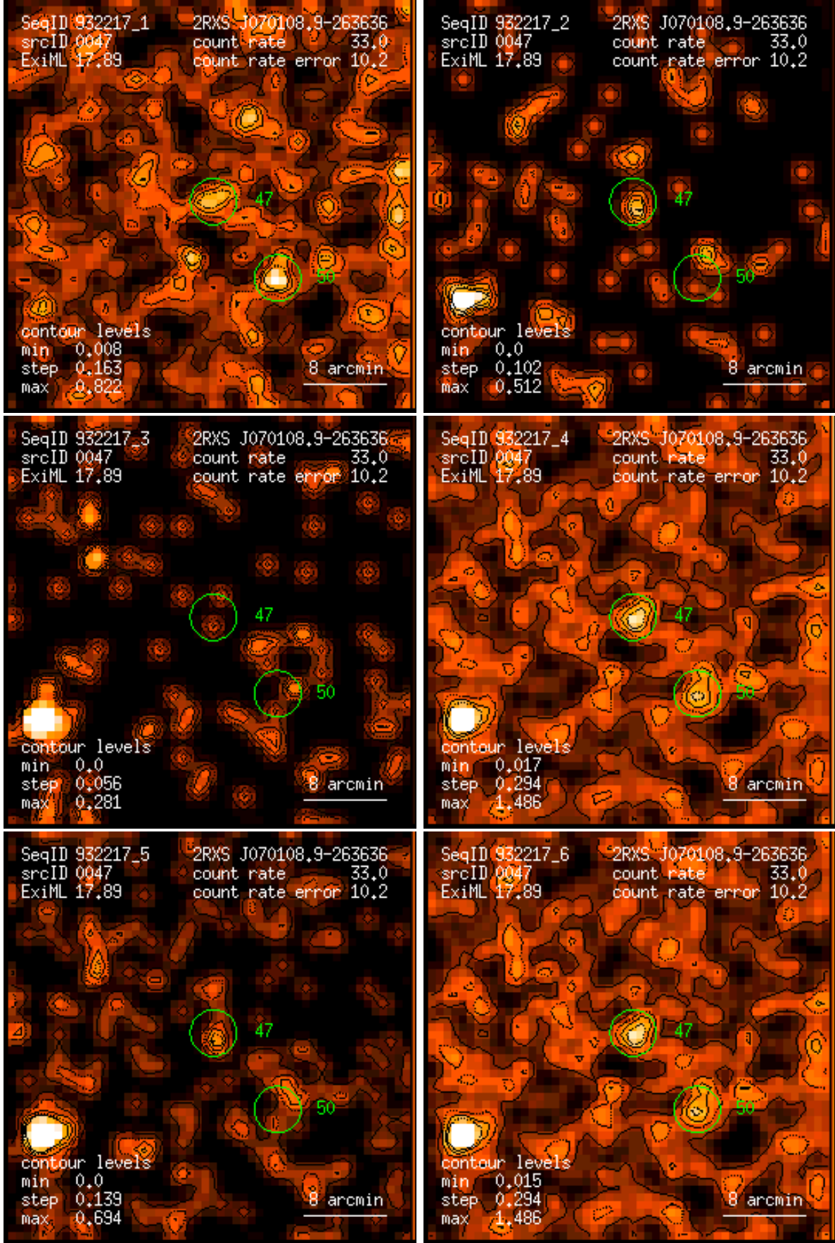
Figure 47: RASS 932217: detection 0047: band rate images, Gaussian filter: (1) PSPC channels 11 – 41, (2) 52 – 90, (3) 91 – 201, (4) 11 – 235, (5) 52 – 201, (6) 11 – 201. Broad band rates in counts/ks. Band rate contour levels in counts/ks/arcmin 2 .
