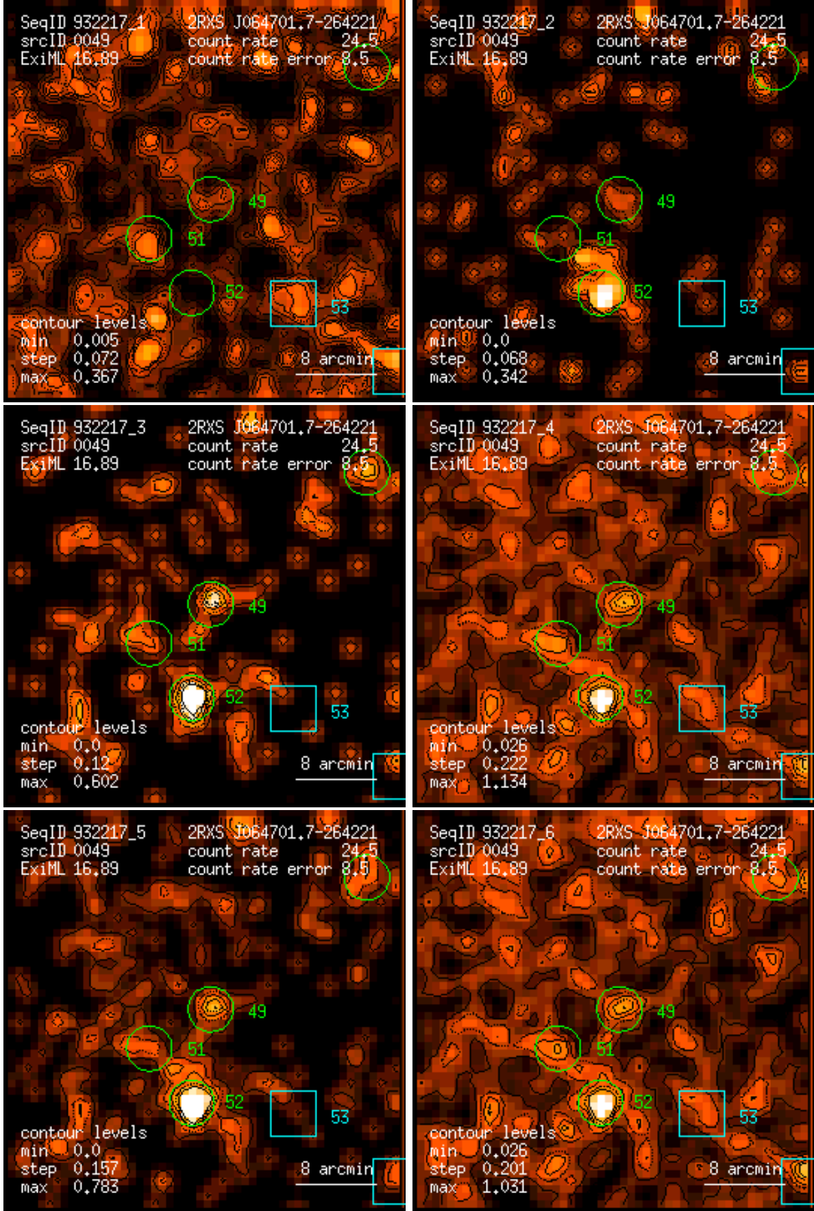
Figure 49: RASS 932217: detection 0049: band rate images, Gaussian filter: (1) PSPC channels 11 – 41, (2) 52 – 90, (3) 91 – 201, (4) 11 – 235, (5) 52 – 201, (6) 11 – 201. Broad band rates in counts/ks. Band rate contour levels in counts/ks/arcmin 2 .
