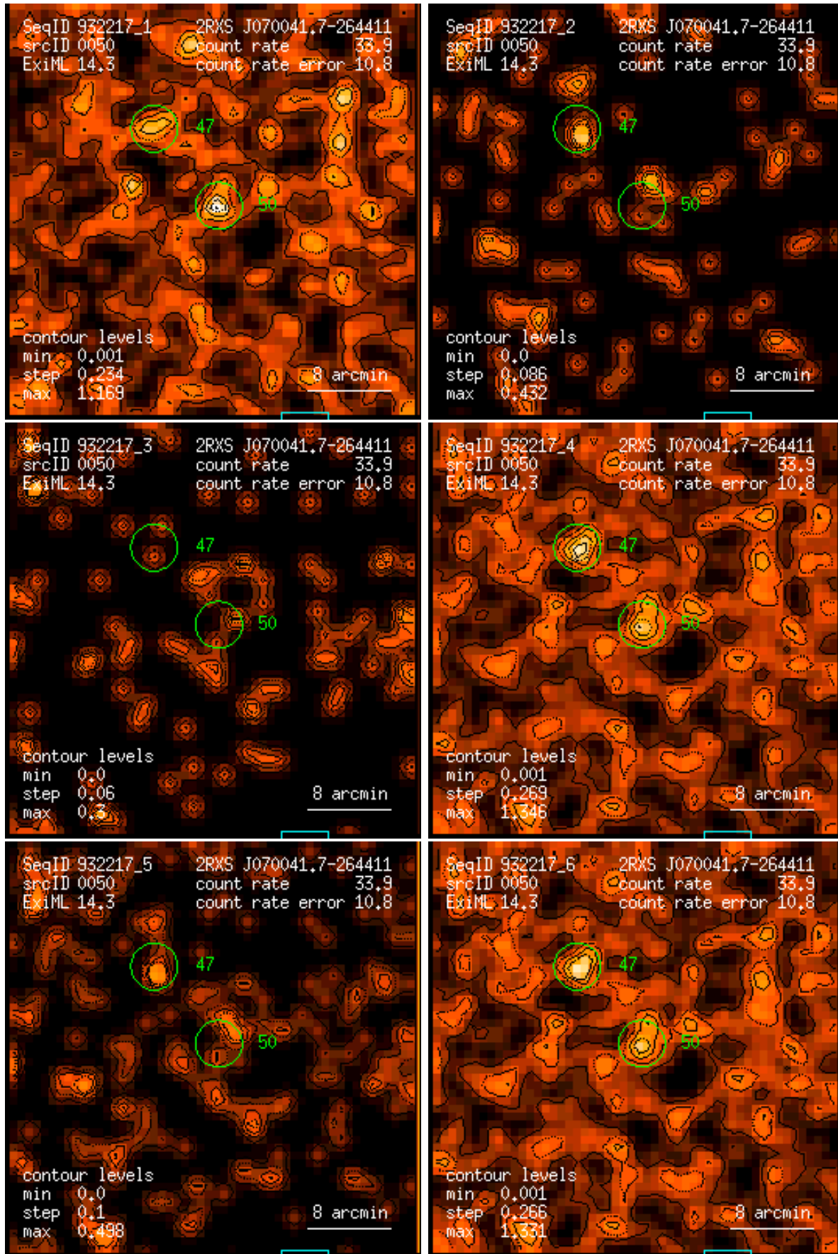
Figure 50: RASS 932217: detection 0050: band rate images, Gaussian filter: (1) PSPC channels 11 – 41, (2) 52 – 90, (3) 91 – 201, (4) 11 – 235, (5) 52 – 201, (6) 11 – 201. Broad band rates in counts/ks. Band rate contour levels in counts/ks/arcmin 2 .
