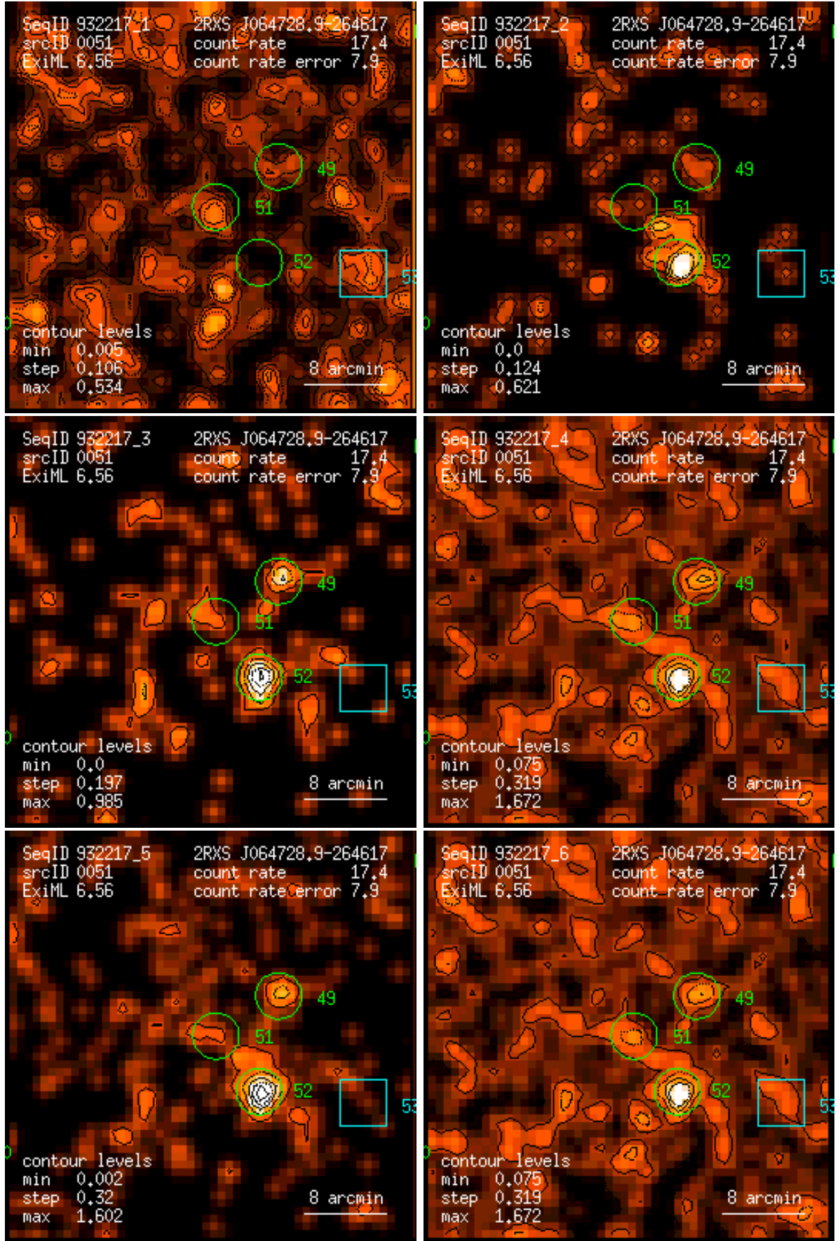
Figure 51: RASS 932217: detection 0051: band rate images, Gaussian filter: (1) PSPC channels 11 – 41, (2) 52 – 90, (3) 91 – 201, (4) 11 – 235, (5) 52 – 201, (6) 11 – 201. Broad band rates in counts/ks. Band rate contour levels in counts/ks/arcmin 2 .
