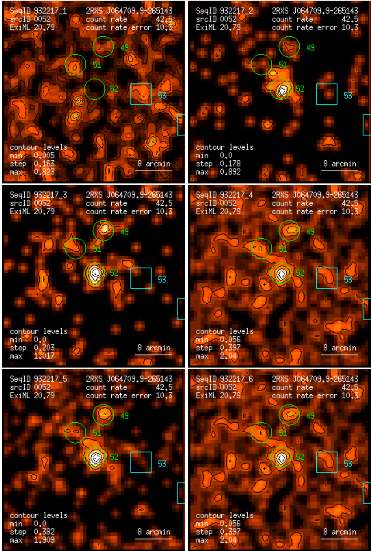
Figure 52: RASS 932217: detection 0052: band rate images, Gaussian filter: (1) PSPC channels 11 – 41, (2) 52 – 90, (3) 91 – 201, (4) 11 – 235, (5) 52 – 201, (6) 11 – 201. Broad band rates in counts/ks. Band rate contour levels in counts/ks/arcmin 2 .
