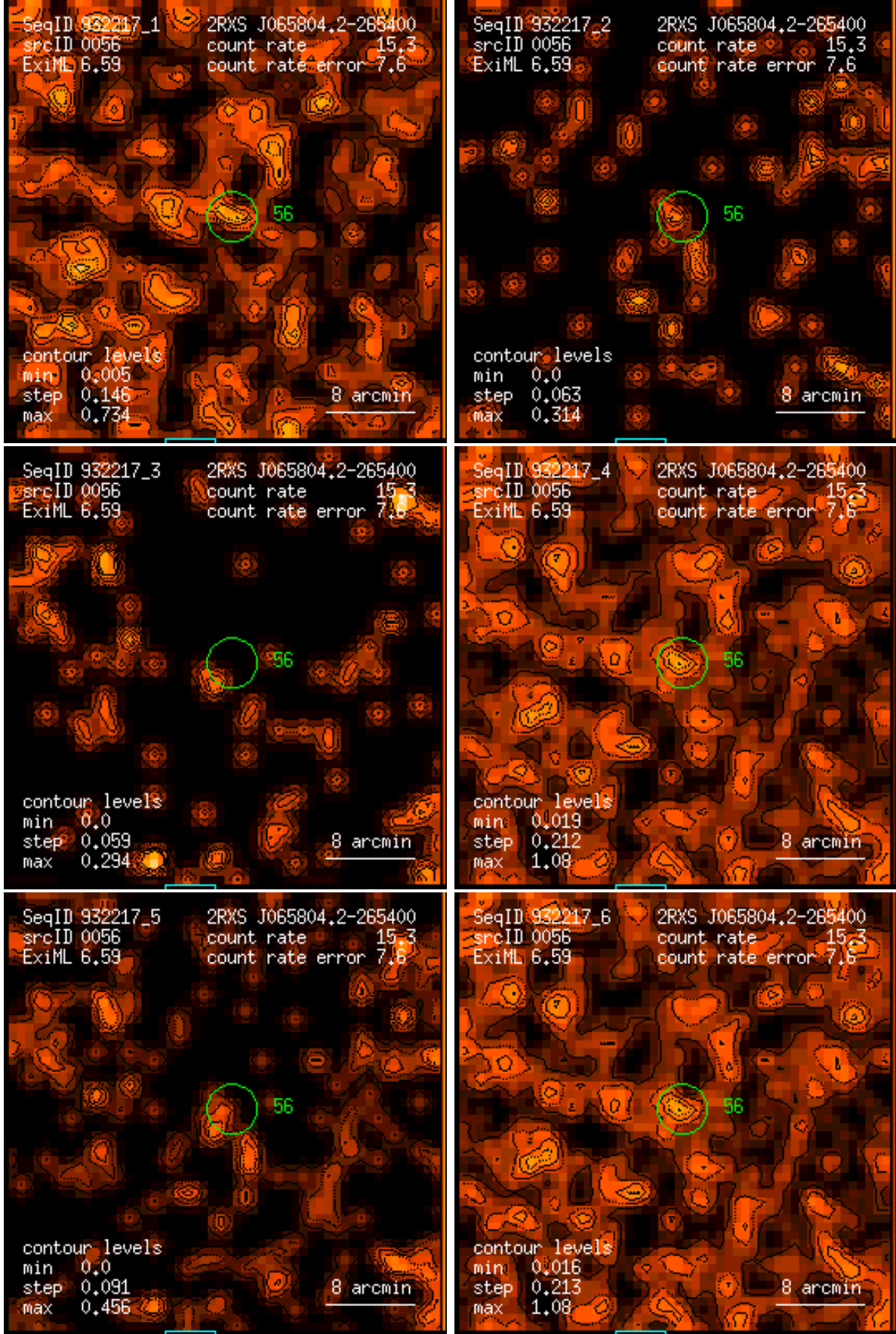
Figure 56: RASS 932217: detection 0056: band rate images, Gaussian filter: (1) PSPC channels 11 – 41, (2) 52 – 90, (3) 91 – 201, (4) 11 – 235, (5) 52 – 201, (6) 11 – 201. Broad band rates in counts/ks. Band rate contour levels in counts/ks/arcmin 2 .
