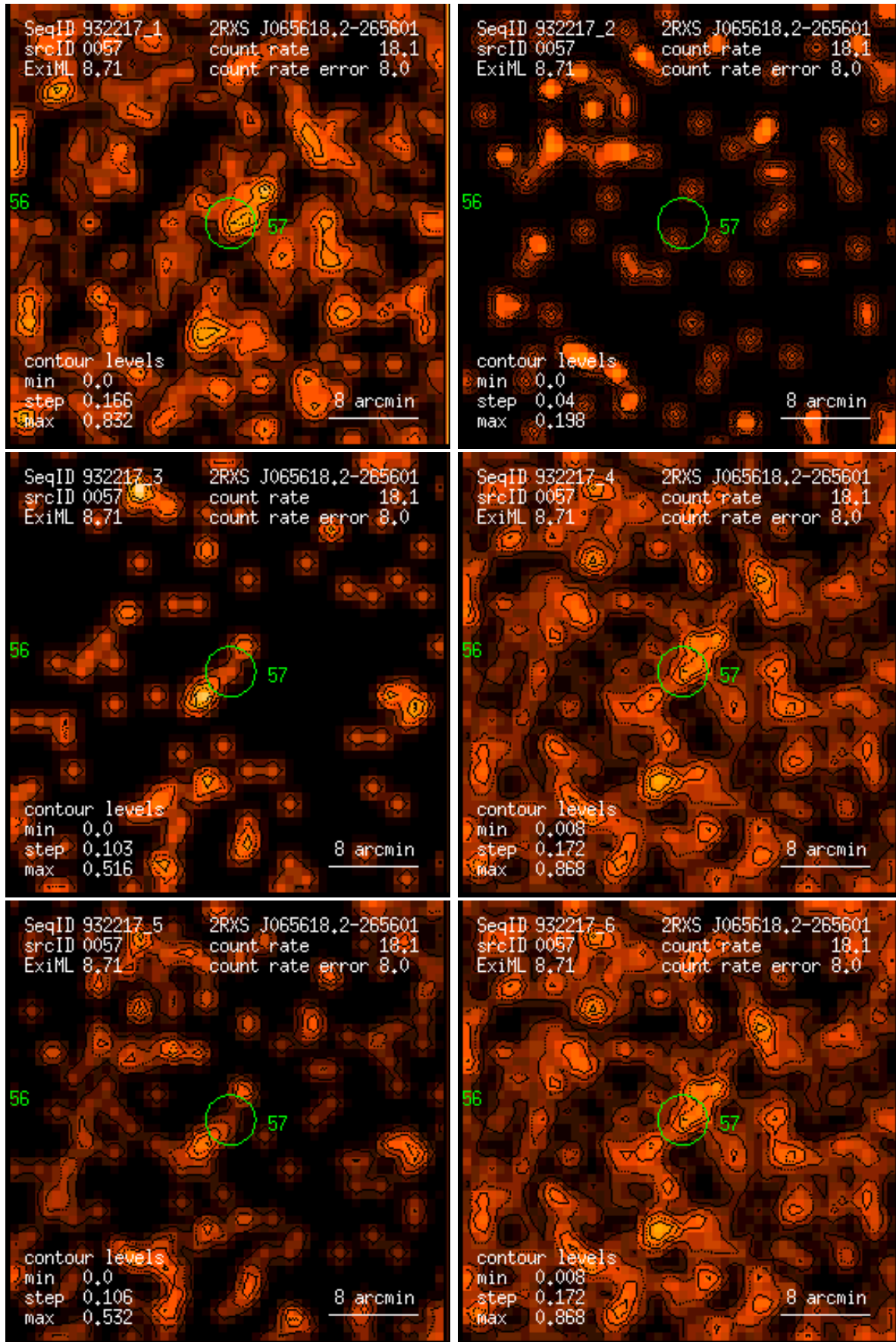
Figure 57: RASS 932217: detection 0057: band rate images, Gaussian filter: (1) PSPC channels 11 – 41, (2) 52 – 90, (3) 91 – 201, (4) 11 – 235, (5) 52 – 201, (6) 11 – 201. Broad band rates in counts/ks. Band rate contour levels in counts/ks/arcmin 2 .
