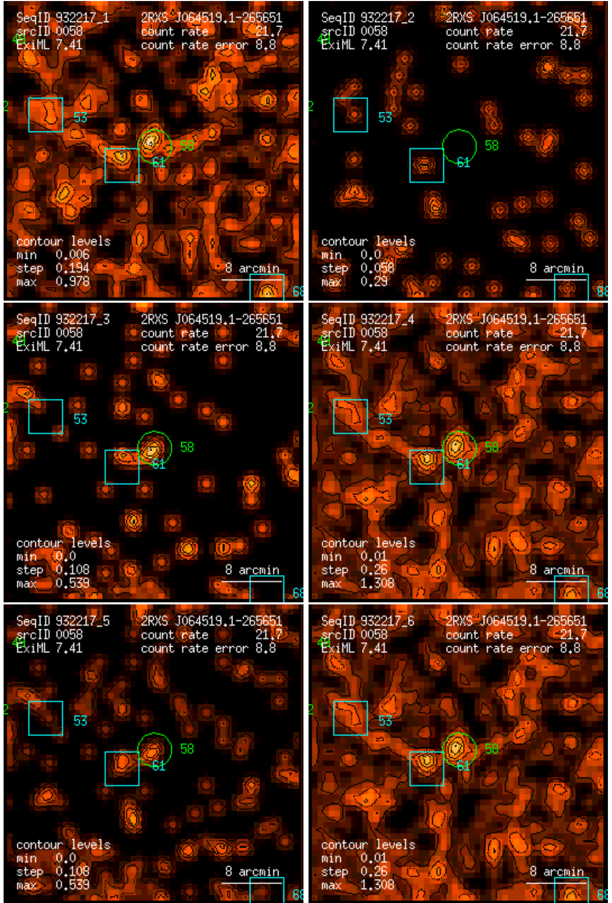
Figure 58: RASS 932217: detection 0058: band rate images, Gaussian filter: (1) PSPC channels 11 – 41, (2) 52 – 90, (3) 91 – 201, (4) 11 – 235, (5) 52 – 201, (6) 11 – 201. Broad band rates in counts/ks. Band rate contour levels in counts/ks/arcmin 2 .
