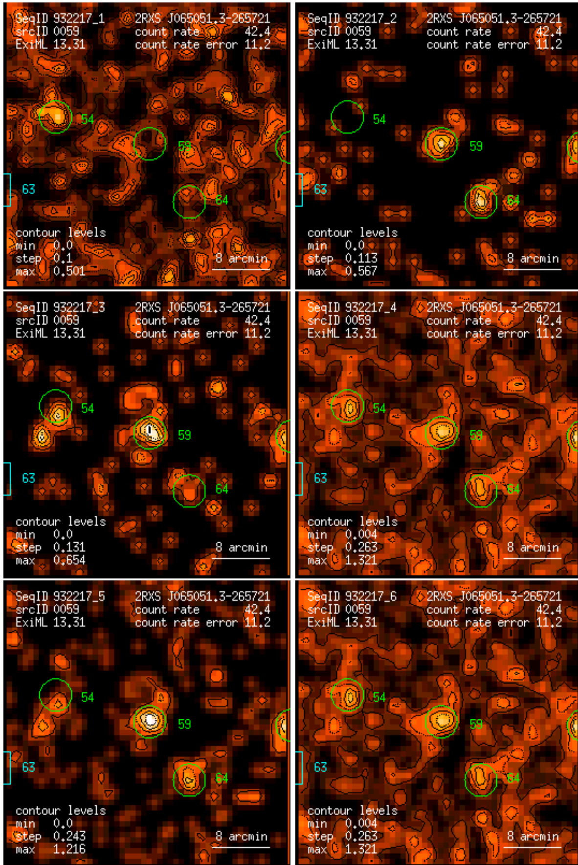
Figure 59: RASS 932217: detection 0059: band rate images, Gaussian filter: (1) PSPC channels 11 – 41, (2) 52 – 90, (3) 91 – 201, (4) 11 – 235, (5) 52 – 201, (6) 11 – 201. Broad band rates in counts/ks. Band rate contour levels in counts/ks/arcmin 2 .
