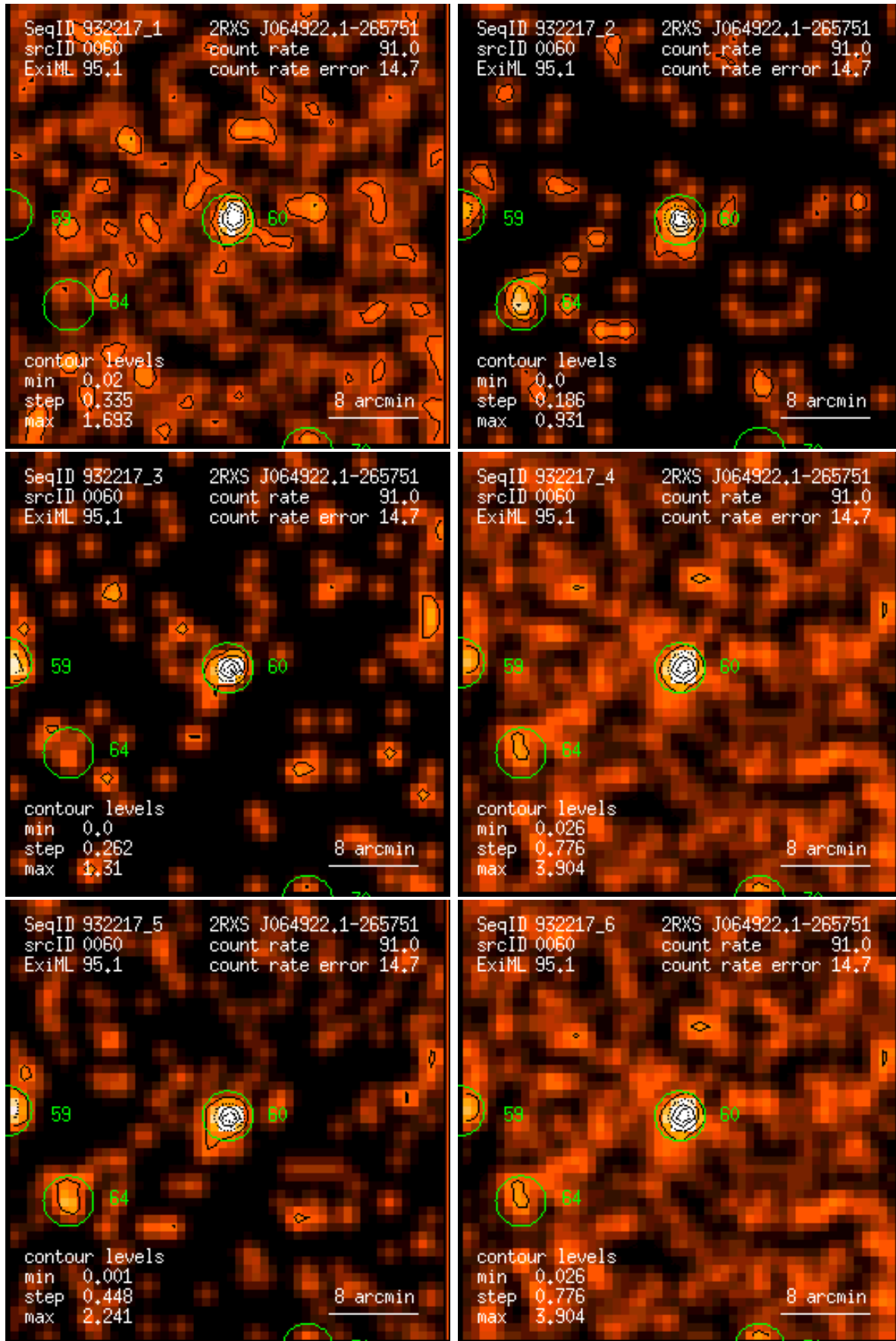
Figure 60: RASS 932217: detection 0060: band rate images, Gaussian filter: (1) PSPC channels 11 – 41, (2) 52 – 90, (3) 91 – 201, (4) 11 – 235, (5) 52 – 201, (6) 11 – 201. Broad band rates in counts/ks. Band rate contour levels in counts/ks/arcmin 2 .
