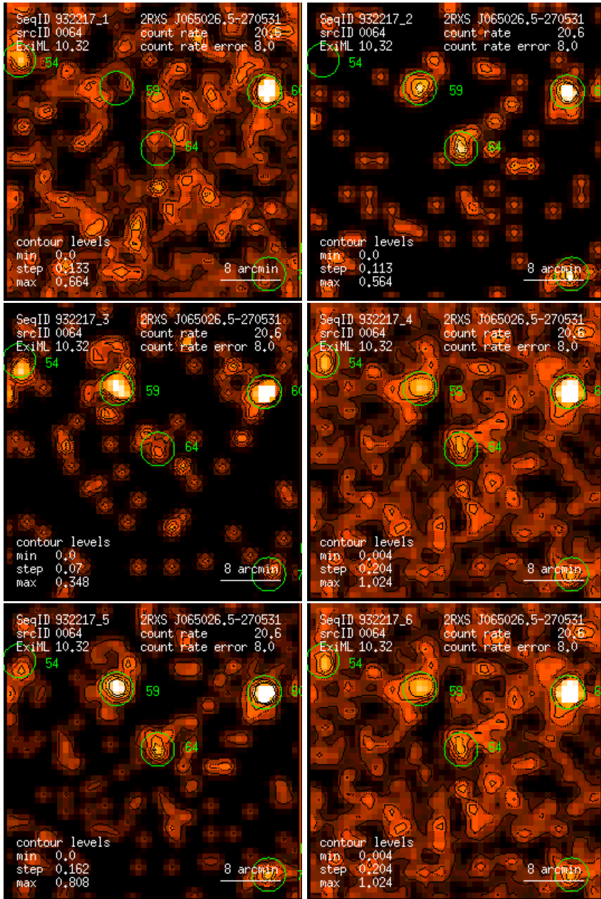
Figure 64: RASS 932217: detection 0064: band rate images, Gaussian filter: (1) PSPC channels 11 – 41, (2) 52 – 90, (3) 91 – 201, (4) 11 – 235, (5) 52 – 201, (6) 11 – 201. Broad band rates in counts/ks. Band rate contour levels in counts/ks/arcmin 2 .
