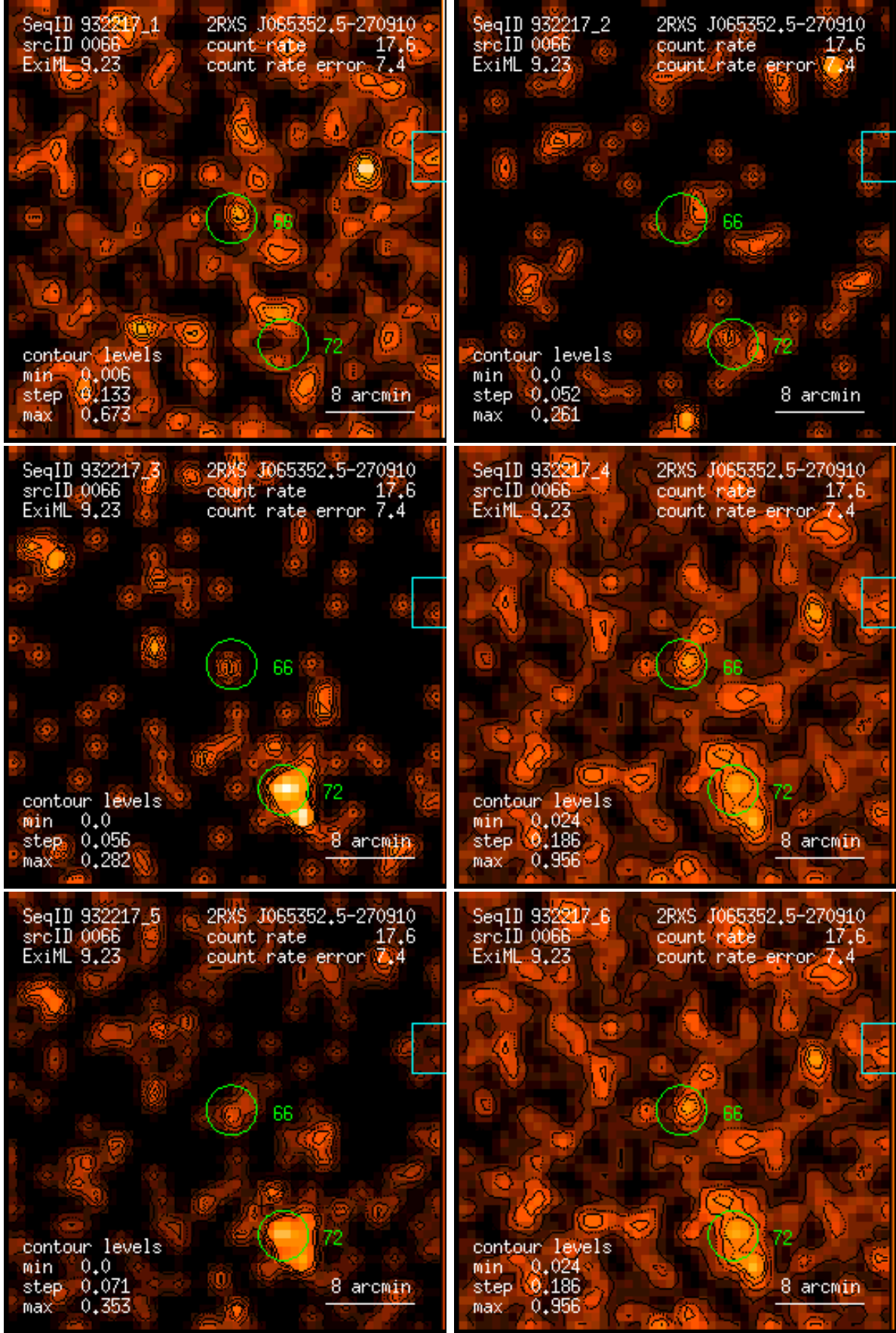
Figure 66: RASS 932217: detection 0066: band rate images, Gaussian filter: (1) PSPC channels 11 – 41, (2) 52 – 90, (3) 91 – 201, (4) 11 – 235, (5) 52 – 201, (6) 11 – 201. Broad band rates in counts/ks. Band rate contour levels in counts/ks/arcmin 2 .
