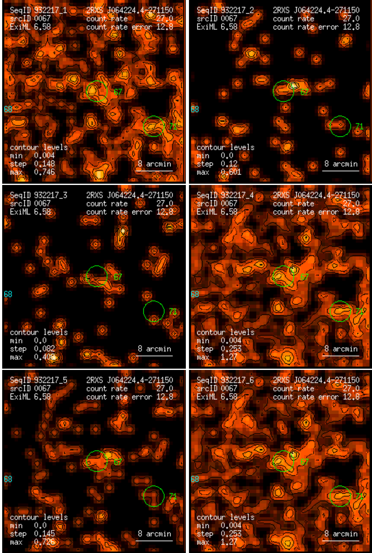
Figure 67: RASS 932217: detection 0067: band rate images, Gaussian filter: (1) PSPC channels 11 – 41, (2) 52 – 90, (3) 91 – 201, (4) 11 – 235, (5) 52 – 201, (6) 11 – 201. Broad band rates in counts/ks. Band rate contour levels in counts/ks/arcmin 2 .
