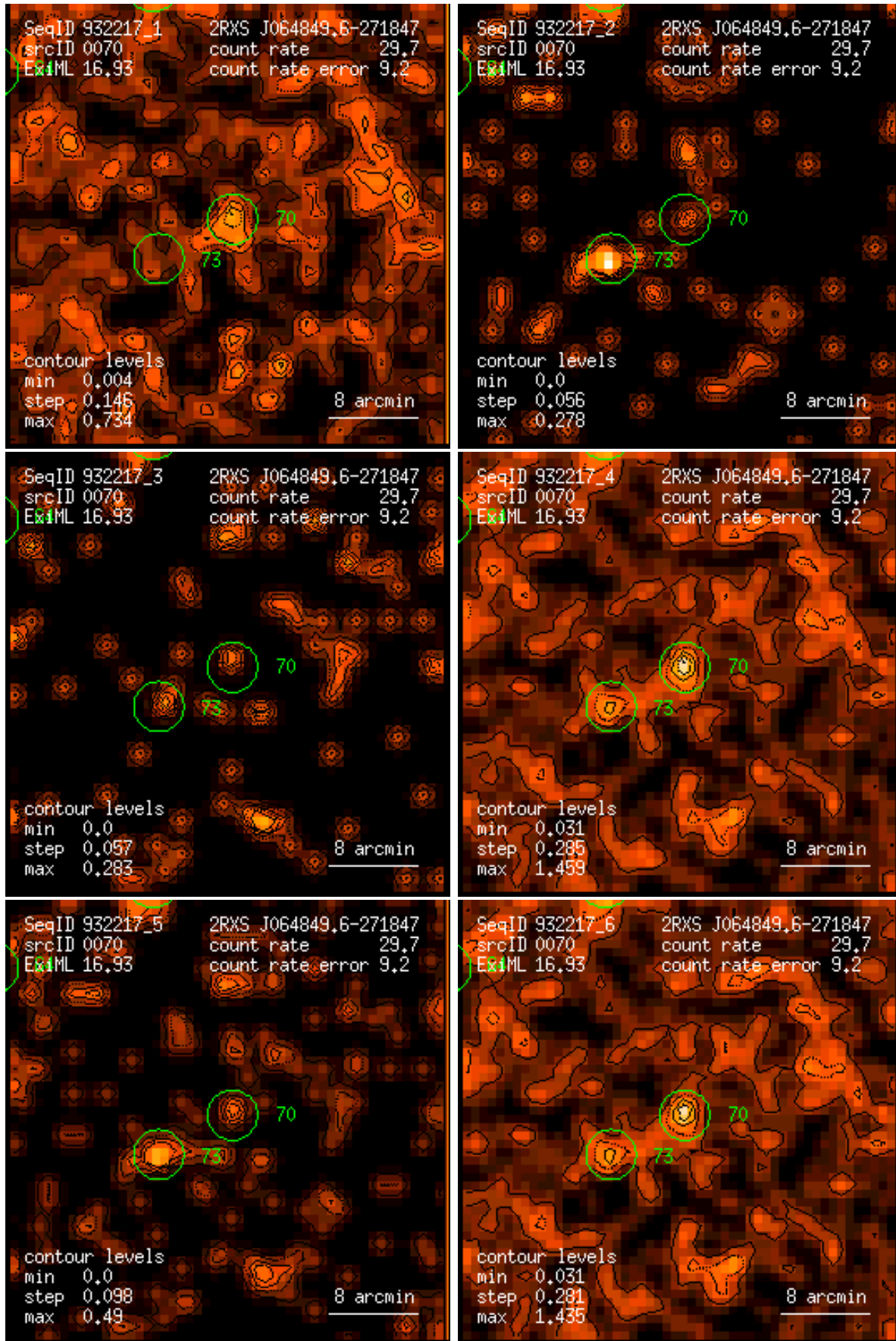
Figure 70: RASS 932217: detection 0070: band rate images, Gaussian filter: (1) PSPC channels 11 – 41, (2) 52 – 90, (3) 91 – 201, (4) 11 – 235, (5) 52 – 201, (6) 11 – 201. Broad band rates in counts/ks. Band rate contour levels in counts/ks/arcmin 2 .
