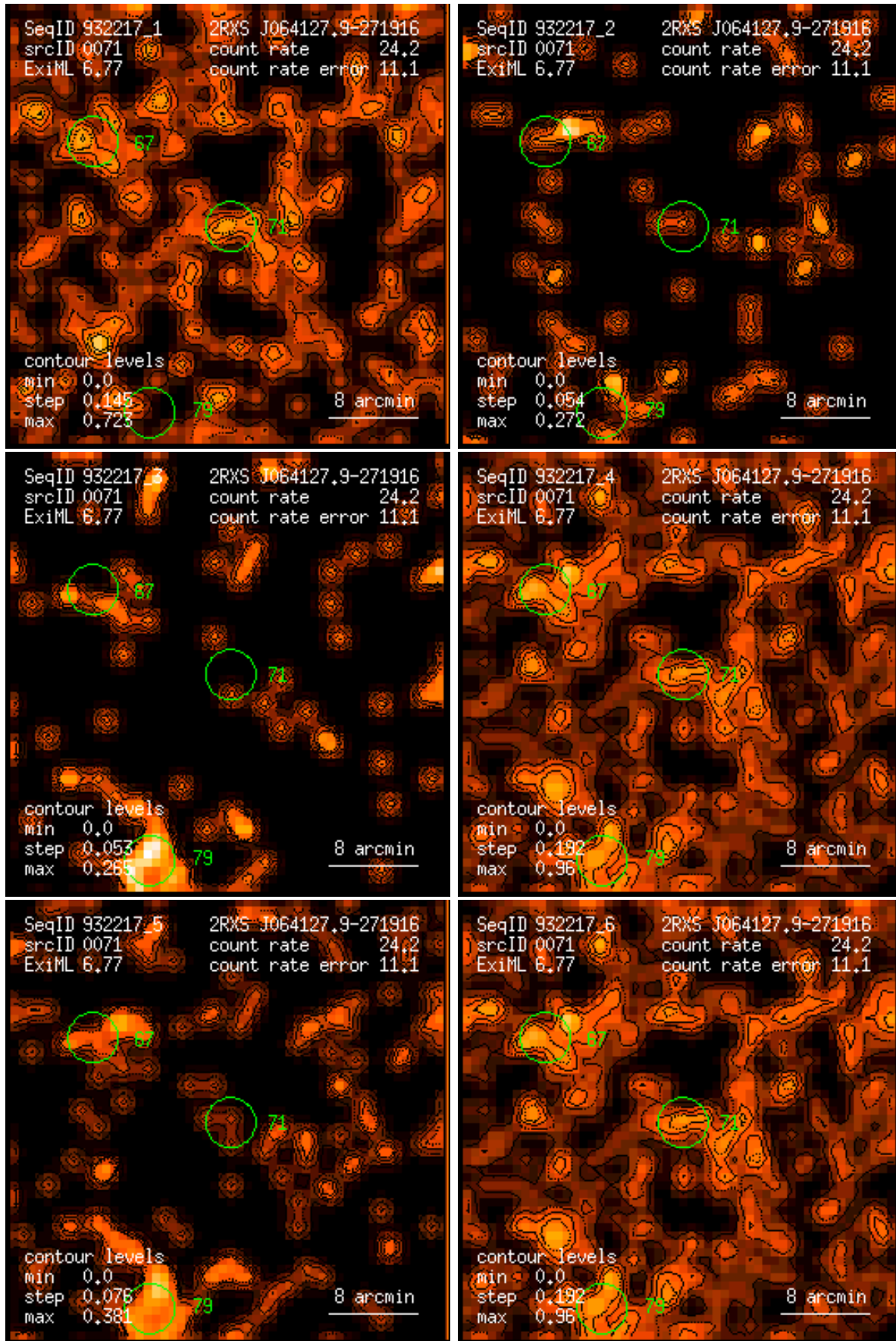
Figure 71: RASS 932217: detection 0071: band rate images, Gaussian filter: (1) PSPC channels 11 – 41, (2) 52 – 90, (3) 91 – 201, (4) 11 – 235, (5) 52 – 201, (6) 11 – 201. Broad band rates in counts/ks. Band rate contour levels in counts/ks/arcmin 2 .
