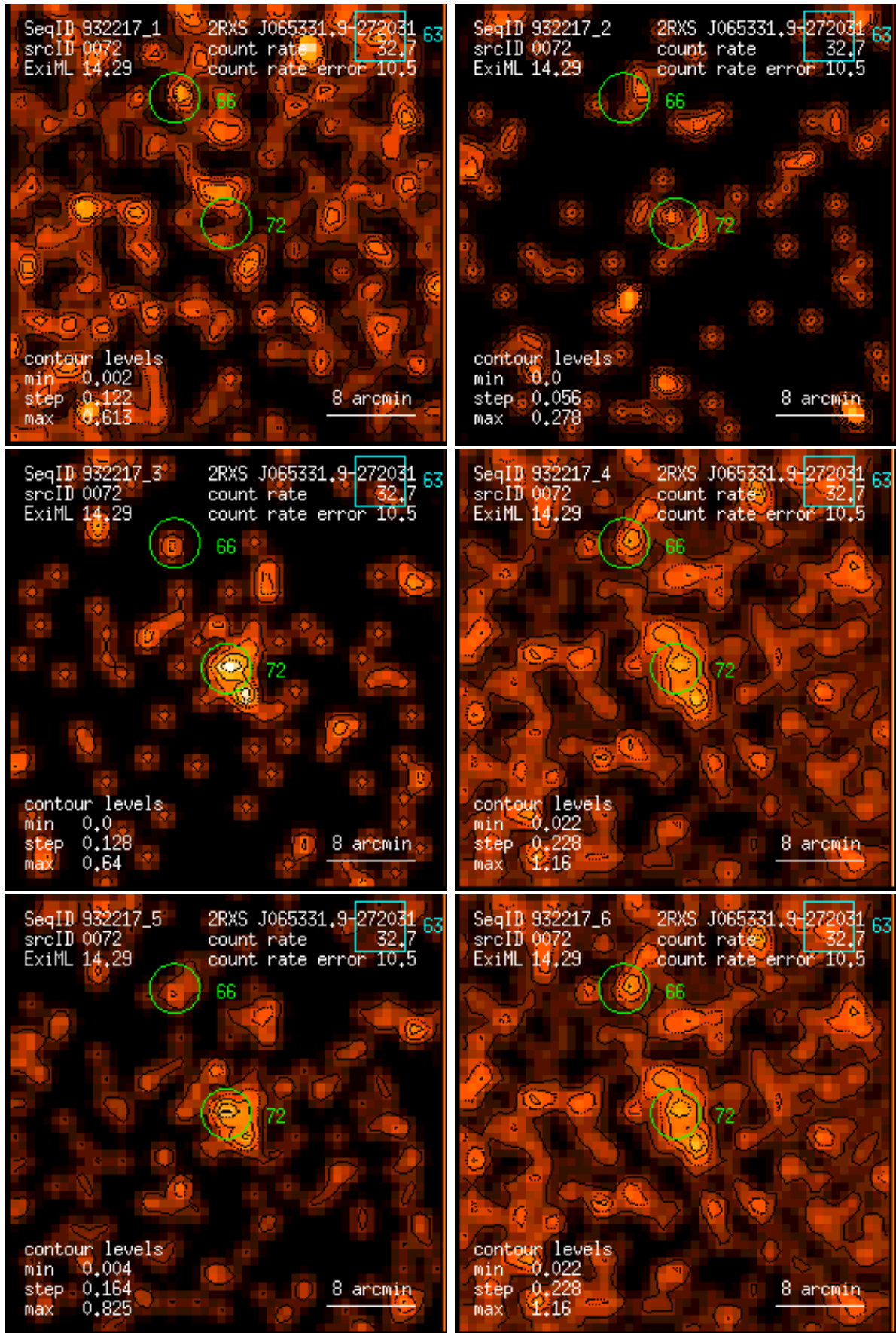
Figure 72: RASS 932217: detection 0072: band rate images, Gaussian filter: (1) PSPC channels 11 – 41, (2) 52 – 90, (3) 91 – 201, (4) 11 – 235, (5) 52 – 201, (6) 11 – 201. Broad band rates in counts/ks. Band rate contour levels in counts/ks/arcmin 2 .
