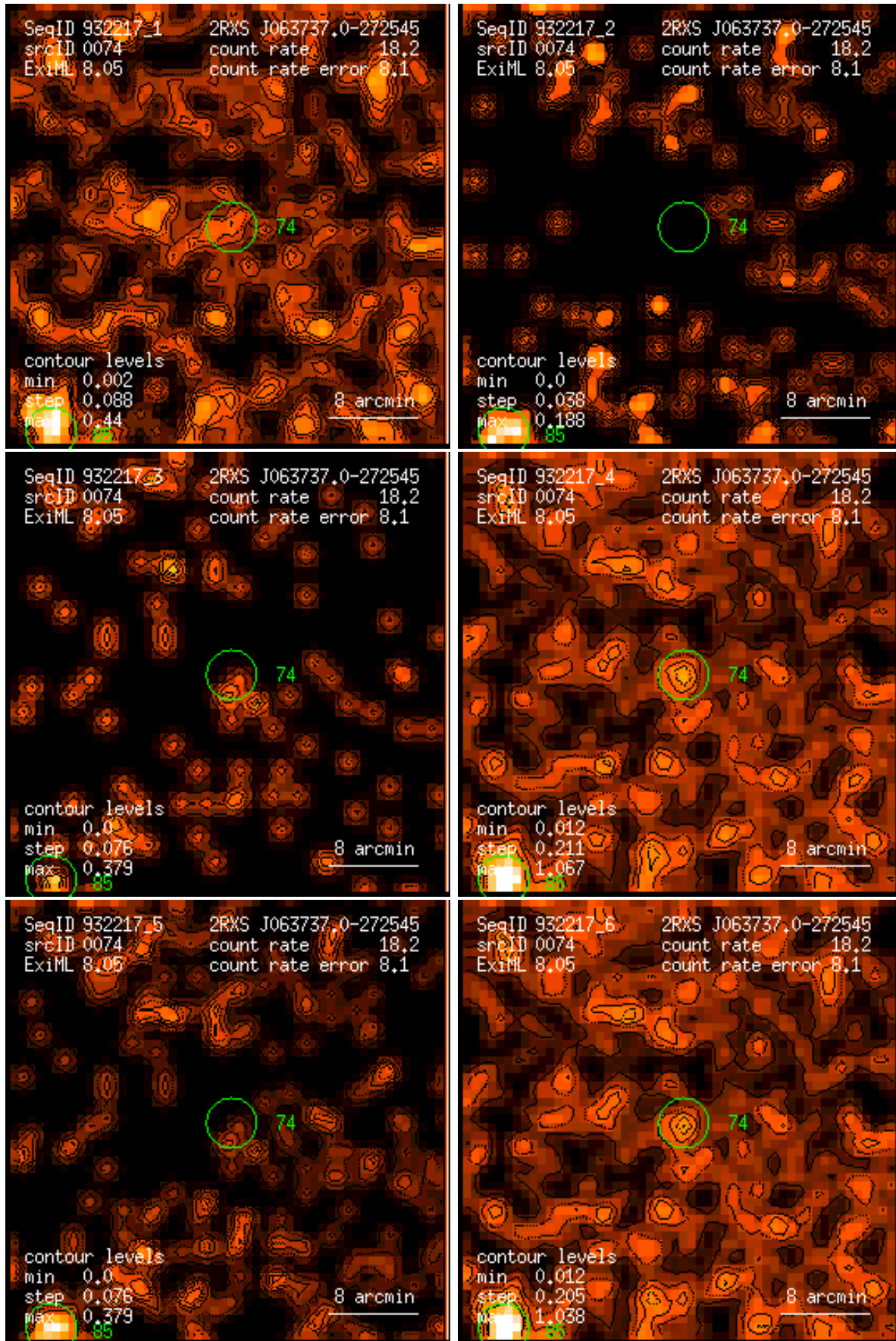
Figure 74: RASS 932217: detection 0074: band rate images, Gaussian filter: (1) PSPC channels 11 – 41, (2) 52 – 90, (3) 91 – 201, (4) 11 – 235, (5) 52 – 201, (6) 11 – 201. Broad band rates in counts/ks. Band rate contour levels in counts/ks/arcmin 2 .
