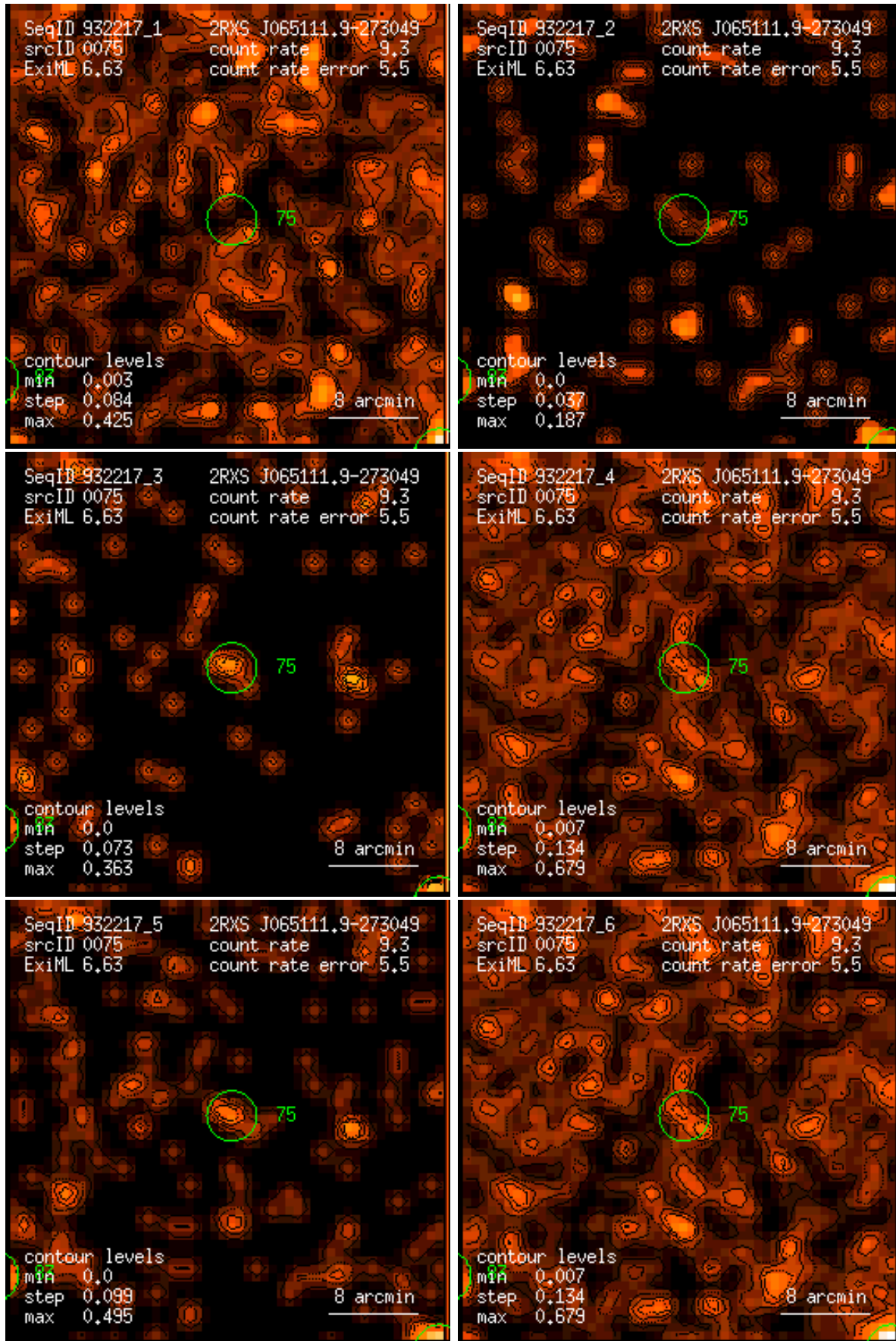
Figure 75: RASS 932217: detection 0075: band rate images, Gaussian filter: (1) PSPC channels 11 – 41, (2) 52 – 90, (3) 91 – 201, (4) 11 – 235, (5) 52 – 201, (6) 11 – 201. Broad band rates in counts/ks. Band rate contour levels in counts/ks/arcmin 2 .
