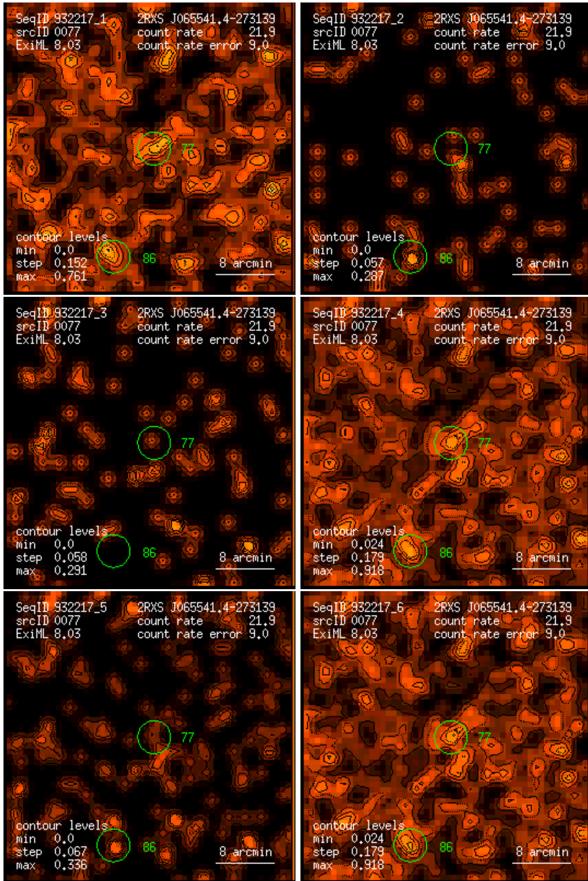
Figure 77: RASS 932217: detection 0077: band rate images, Gaussian filter: (1) PSPC channels 11 – 41, (2) 52 – 90, (3) 91 – 201, (4) 11 – 235, (5) 52 – 201, (6) 11 – 201. Broad band rates in counts/ks. Band rate contour levels in counts/ks/arcmin 2 .
