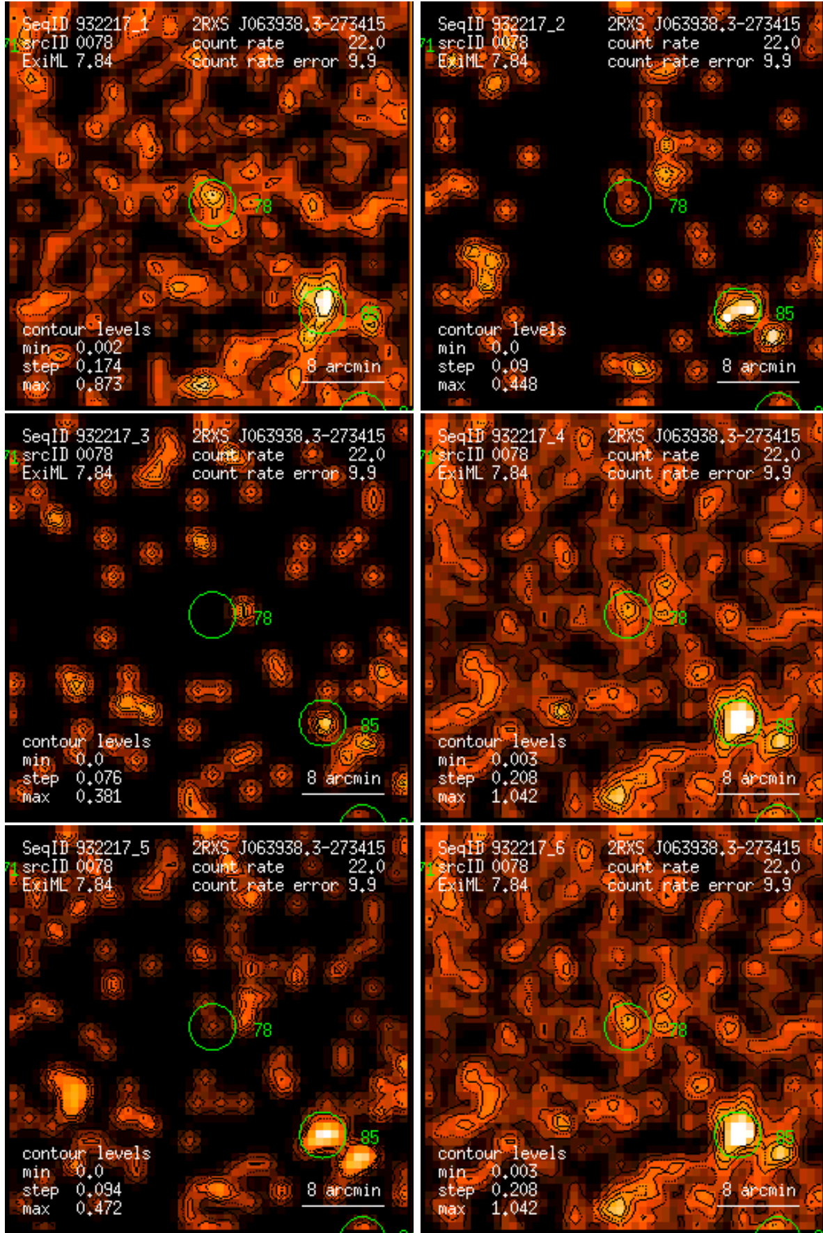
Figure 78: RASS 932217: detection 0078: band rate images, Gaussian filter: (1) PSPC channels 11 – 41, (2) 52 – 90, (3) 91 – 201, (4) 11 – 235, (5) 52 – 201, (6) 11 – 201. Broad band rates in counts/ks. Band rate contour levels in counts/ks/arcmin 2 .
