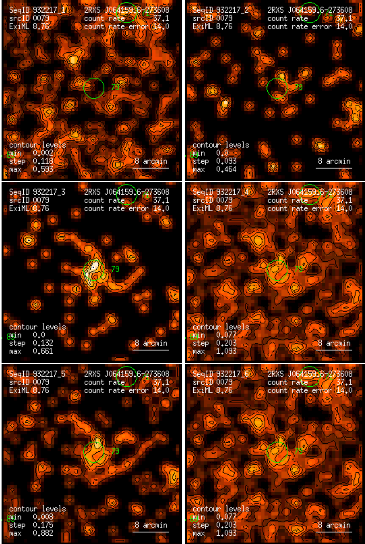
Figure 79: RASS 932217: detection 0079: band rate images, Gaussian filter: (1) PSPC channels 11 – 41, (2) 52 – 90, (3) 91 – 201, (4) 11 – 235, (5) 52 – 201, (6) 11 – 201. Broad band rates in counts/ks. Band rate contour levels in counts/ks/arcmin 2 .
