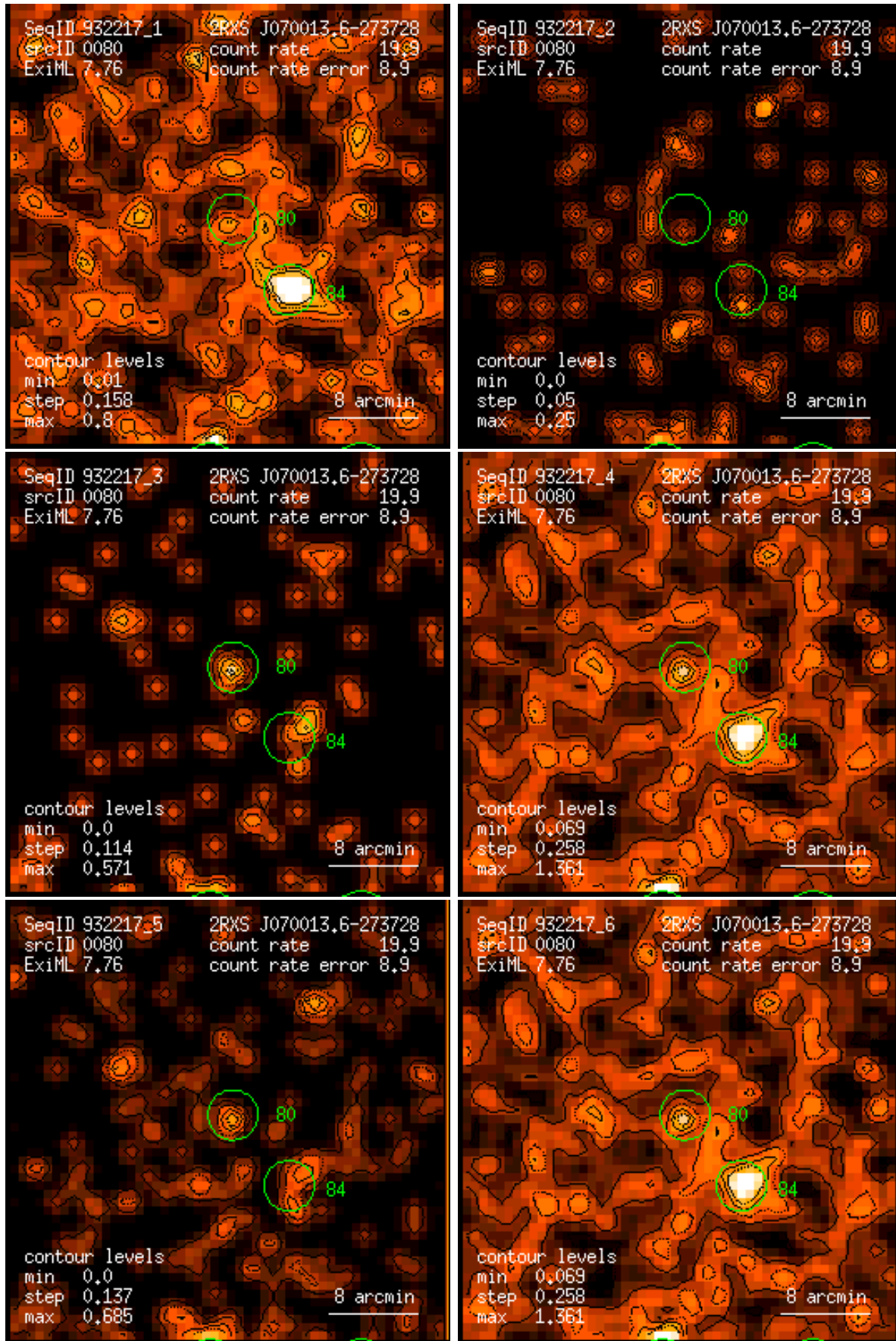
Figure 80: RASS 932217: detection 0080: band rate images, Gaussian filter: (1) PSPC channels 11 – 41, (2) 52 – 90, (3) 91 – 201, (4) 11 – 235, (5) 52 – 201, (6) 11 – 201. Broad band rates in counts/ks. Band rate contour levels in counts/ks/arcmin 2 .
