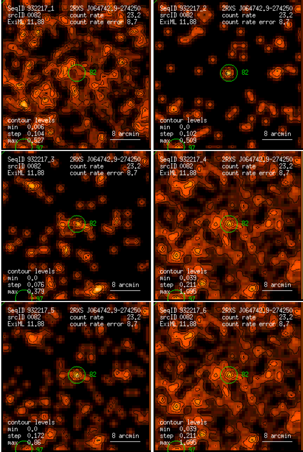
Figure 82: RASS 932217: detection 0082: band rate images, Gaussian filter: (1) PSPC channels 11 – 41, (2) 52 – 90, (3) 91 – 201, (4) 11 – 235, (5) 52 – 201, (6) 11 – 201. Broad band rates in counts/ks. Band rate contour levels in counts/ks/arcmin 2 .
