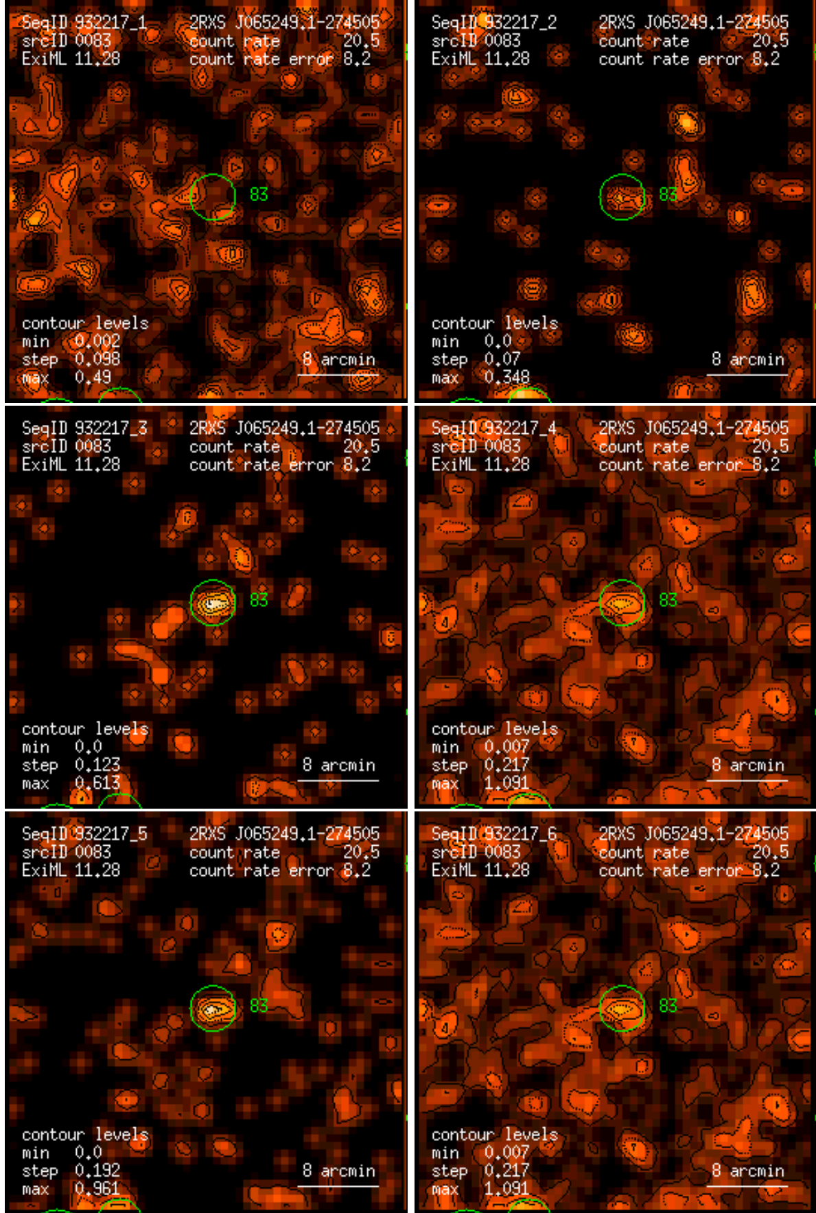
Figure 83: RASS 932217: detection 0083: band rate images, Gaussian filter: (1) PSPC channels 11 – 41, (2) 52 – 90, (3) 91 – 201, (4) 11 – 235, (5) 52 – 201, (6) 11 – 201. Broad band rates in counts/ks. Band rate contour levels in counts/ks/arcmin 2 .
