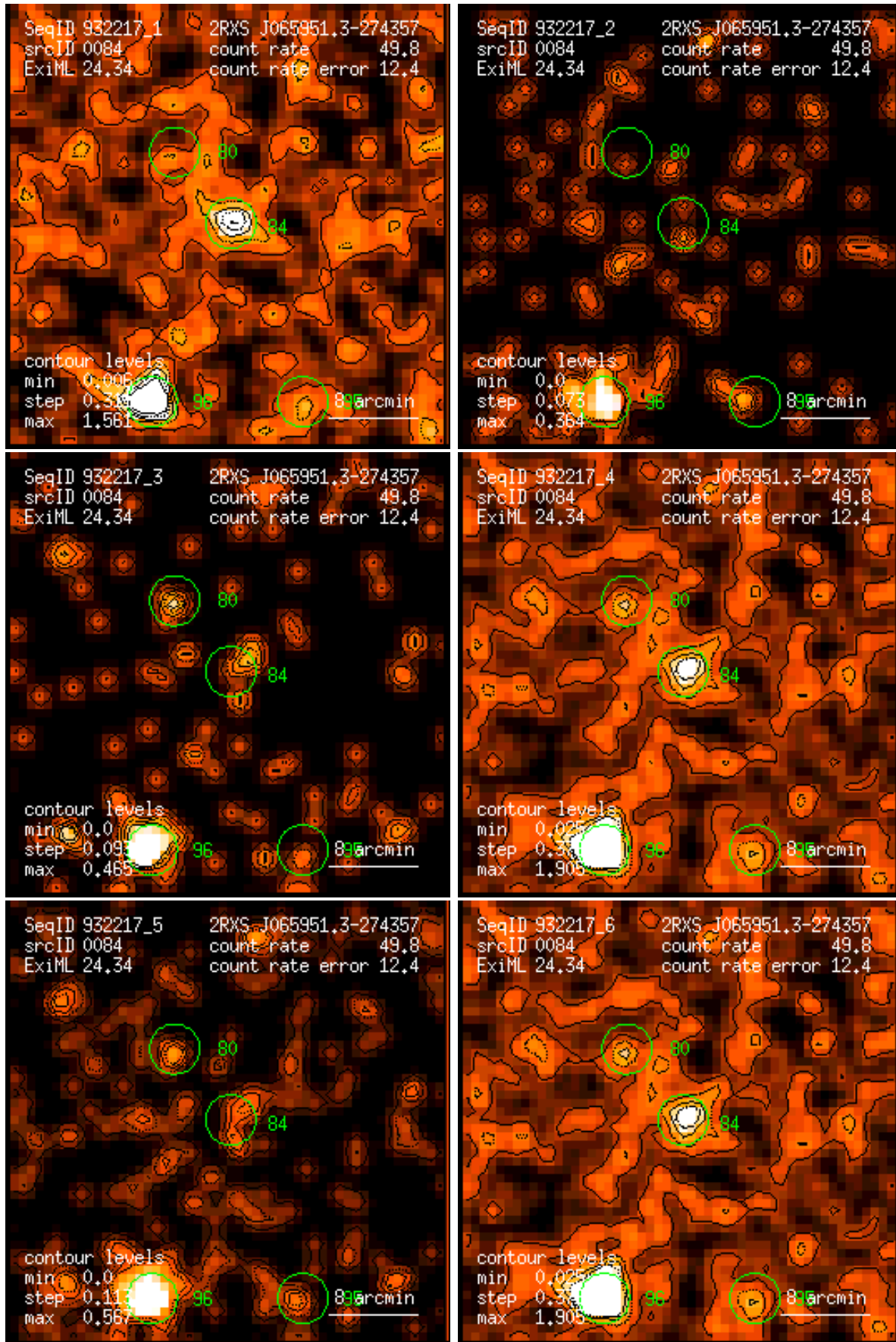
Figure 84: RASS 932217: detection 0084: band rate images, Gaussian filter: (1) PSPC channels 11 – 41, (2) 52 – 90, (3) 91 – 201, (4) 11 – 235, (5) 52 – 201, (6) 11 – 201. Broad band rates in counts/ks. Band rate contour levels in counts/ks/arcmin 2 .
