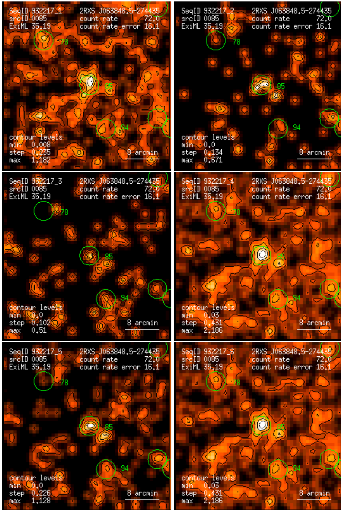
Figure 85: RASS 932217: detection 0085: band rate images, Gaussian filter: (1) PSPC channels 11 – 41, (2) 52 – 90, (3) 91 – 201, (4) 11 – 235, (5) 52 – 201, (6) 11 – 201. Broad band rates in counts/ks. Band rate contour levels in counts/ks/arcmin 2 .
