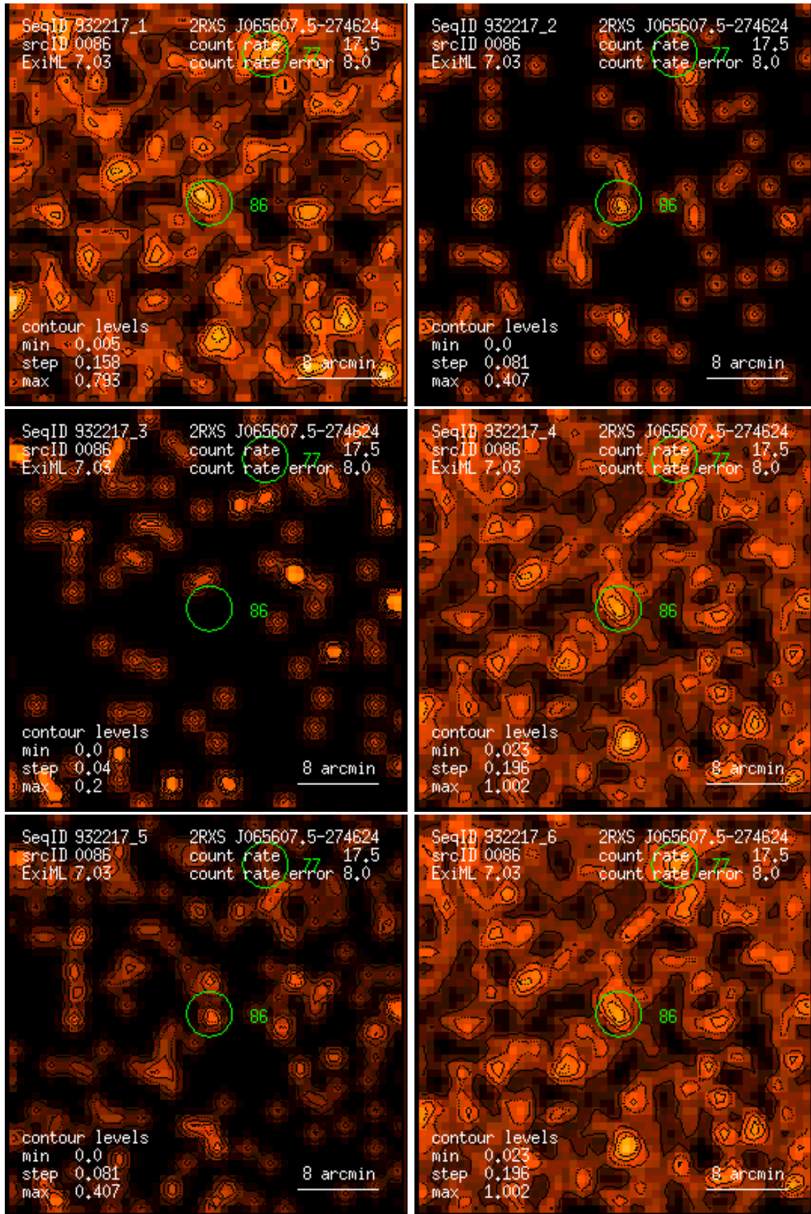
Figure 86: RASS 932217: detection 0086: band rate images, Gaussian filter: (1) PSPC channels 11 – 41, (2) 52 – 90, (3) 91 – 201, (4) 11 – 235, (5) 52 – 201, (6) 11 – 201. Broad band rates in counts/ks. Band rate contour levels in counts/ks/arcmin 2 .
