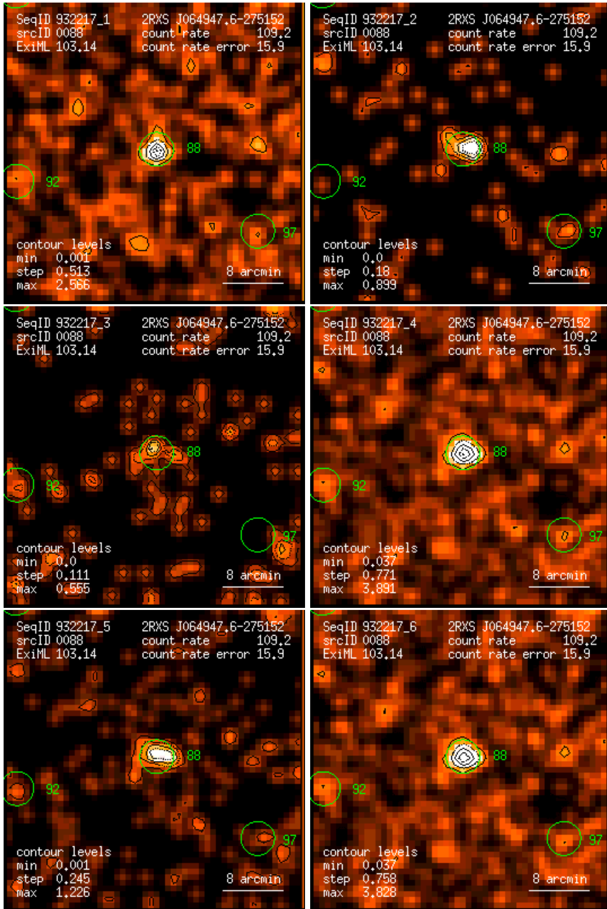
Figure 88: RASS 932217: detection 0088: band rate images, Gaussian filter: (1) PSPC channels 11 – 41, (2) 52 – 90, (3) 91 – 201, (4) 11 – 235, (5) 52 – 201, (6) 11 – 201. Broad band rates in counts/ks. Band rate contour levels in counts/ks/arcmin 2 .
