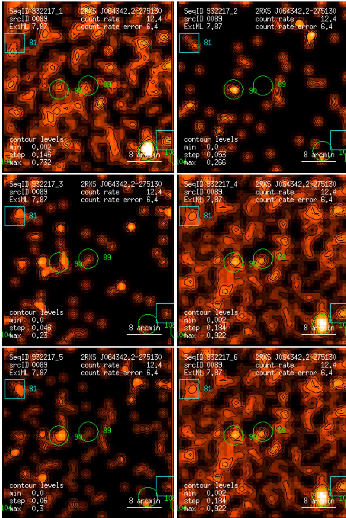
Figure 89: RASS 932217: detection 0089: band rate images, Gaussian filter: (1) PSPC channels 11 – 41, (2) 52 – 90, (3) 91 – 201, (4) 11 – 235, (5) 52 – 201, (6) 11 – 201. Broad band rates in counts/ks. Band rate contour levels in counts/ks/arcmin 2 .
